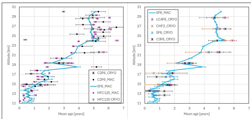
Figure 6. Left: Mean ages of air versus altitude as derived from tropospheric trends and stratospheric mole fraction as available from the MAC and the CRYO samplers for C_2F_6 , SF_6 (MAC only), and HFC-125. Right: The same but for C_3F_8 , SF_6 (including CRYO), c-C_4F_8 , and CHF_3 . All SF_6 -based ages have been sink -corrected according to Garny et al. (2024a).
