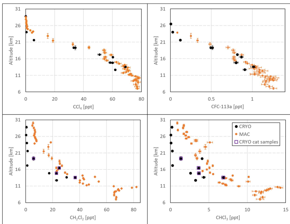
Figure 5. The same as in Figure 3 but for \text{CCl}_4 (top left), \text{CFC-113a} (top right), \text{CH}_2\text{Cl}_2 (lower left), and \text{CHCl}_3 (lower right).
