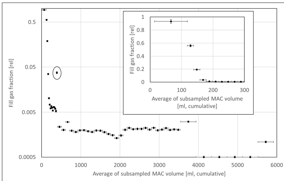
Figure 2: Cumulated fill gas fraction contained in the subsamples collected from the MAC as a function of the cumulative subsampled volume (averaged per sample) as determined from the content of PFTEA. The inset illustrates the rapid drop in fill gas fraction over the first 10 samples on a non-logarithmic scale. For four samples the PFTEA signal was too small to be quantified, these are shown as the detection limit (0.0005). Vertical error bars depict the analytically determined fraction uncertainty, whereas horizontal error bars refer to the sample size. The circled data point shows unusually high PFTEA, which is likely caused by the subsampling procedure. Further details can be found in Section 3.1.
