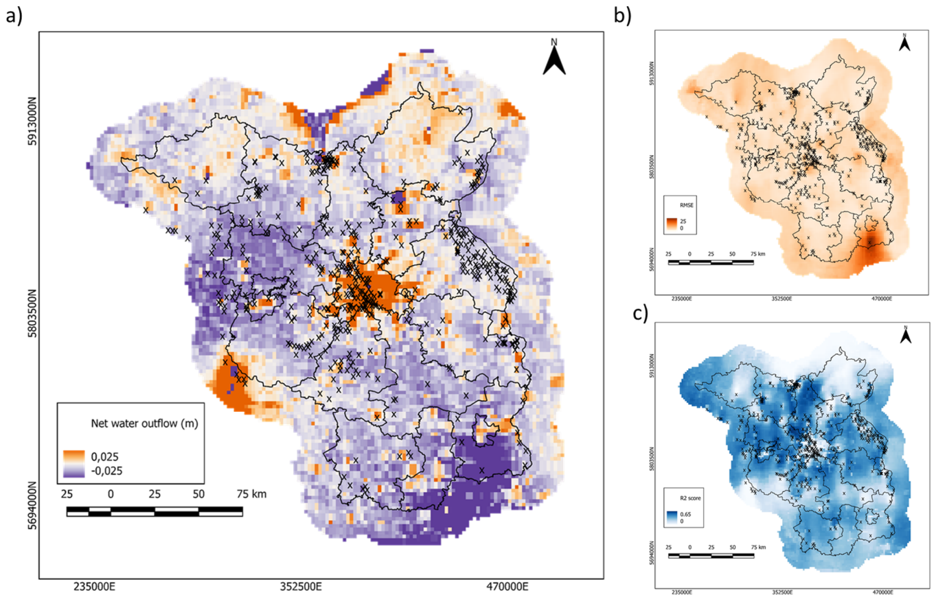
325 Figure 4. a) Estimated net water outflow from the water balance model. Blue color marks areas with water flowing in (water deficit, discharge areas), orange colors mark areas with water flowing out (water surplus, recharge areas), b) RMSE misfits of the calibrated water balance model, c) r2score of the calibrated water balance model.
