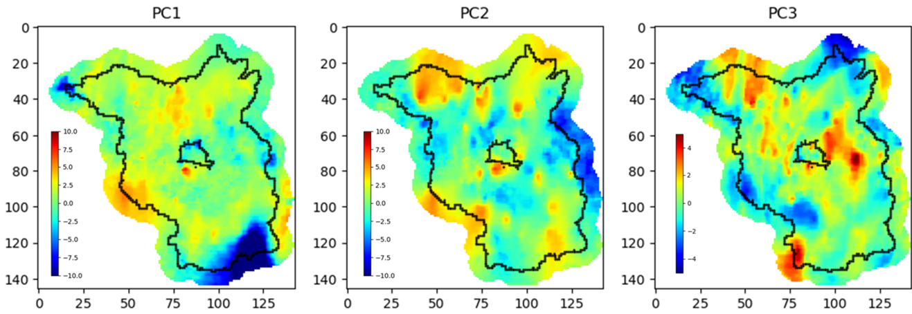
435 Figure 6: Results of the principal component analysis a) 1 st PC, b) 2 nd PC, c) 3 rd PC.
