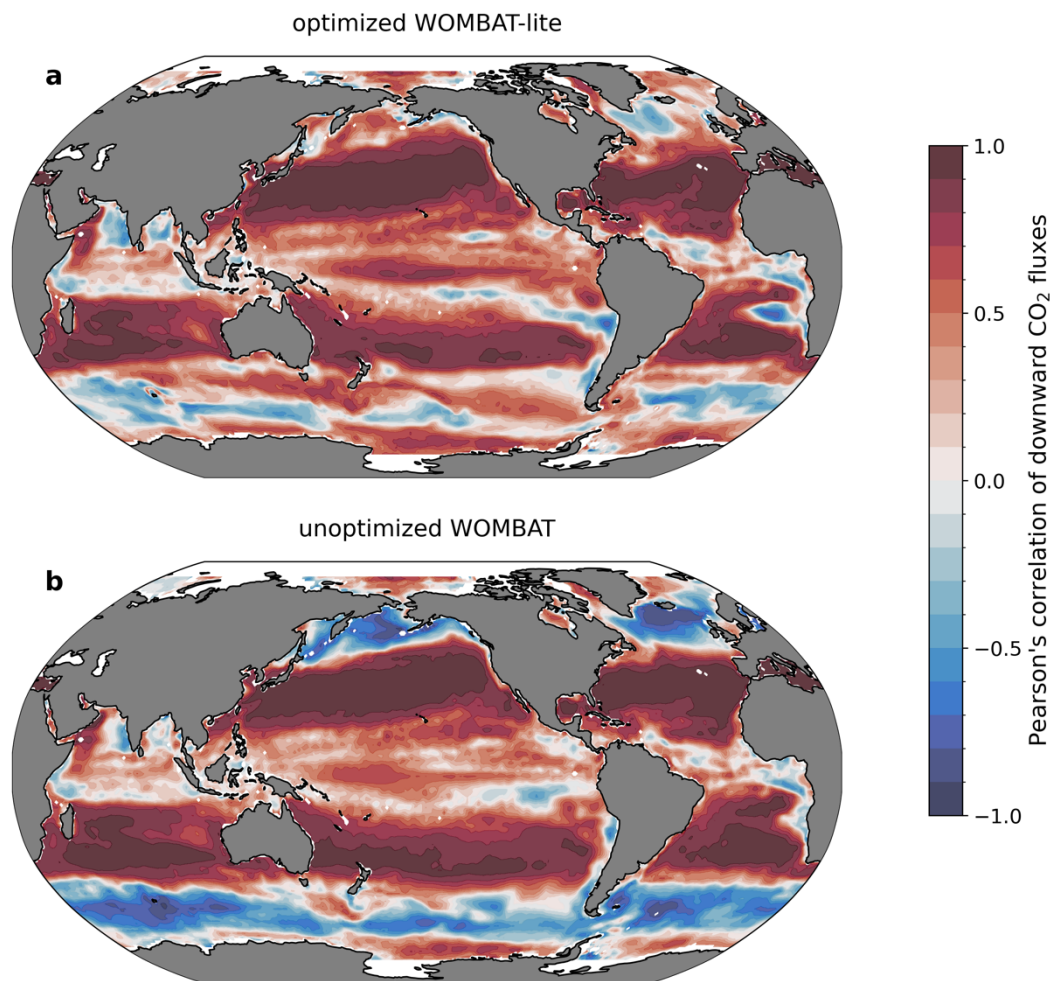
655 Figure 11. Temporal correlations in monthly CO 2 fluxes with an observation product (Chau et al., 2022). (a), optimised WOMBAT- lite and (b), unoptimized, previous WOMBAT over years 1985 to 2019.
