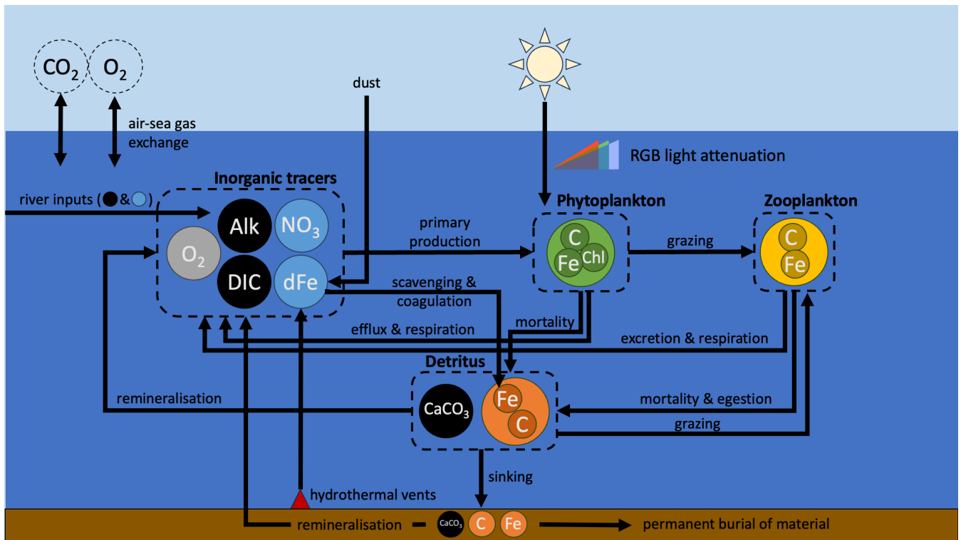
135 Figure 2. Schematic representation of WOMBAT-lite. Tracers and biomass pools are represented by circles of different colours. Black tracers represent the carbon system, blue are inorganic nutrients. Inner circles of C, Chl and Fe within each biomass pool represent the units of carbon, chlorophyll and iron that are explicitly tracked. Major components are grouped within the dashed outlines. Although dissolved inorganic carbon (DIC), alkalinity (Alk) and oxygen (O 2 ) are connected to primary production, they are only affected by it and do not limit 140 primary production of phytoplankton. In contrast, both nitrate (NO 3 ) and dissolved iron (dFe) are biogeochemical tracers whose availability both controls and is affected by phytoplankton growth. Dust and hydrothermal iron input dFe, while rivers input DIC, Alk, NO 3 and dFe. Atmospheric concentrations of carbon dioxide (CO 2 ) and O 2 are not explicitly tracked by the ocean model (dashed circles).
