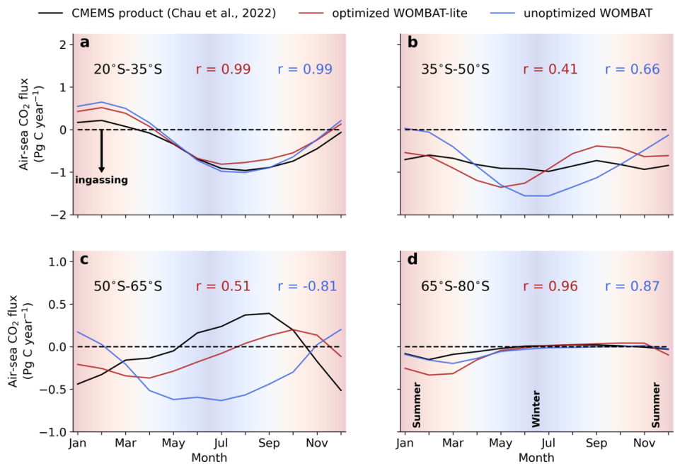
Figure 10. Climatological evolution of the integrated air-sea CO 2 flux over the latitudinal bands in the Southern Oceans averaged over years 1990 to 2010. (a), Observational product from the Copernicus Marine Environmental Monitoring Service (black) are compared with fluxes from WOMBAT-lite (red) and an unoptimized, previous version of WOMBAT (blue) integrated between 20°S-35°S (subtropics). Pearson's correlations are shown for both models. Negative values are net ingassing of CO 2 into the ocean. Background shading denotes the seasonal transition from summer to winter to summer. Panels (b), (c), and (d) are the same as in (a), but integrated within 35°S-50°S for the subtropical-subantarctic transition, 50°S-65°S for the Antarctic Circumpolar Current and 65°S-80°S for Antarctic zone, respectively.
