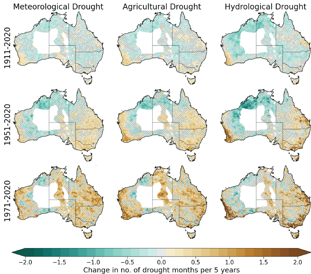
Figure 2: Trends in time under drought for the three traditional drought types and three time periods. The maps show the change in the number of drought months per 5 years during the three time periods. The hatching indicates where the trend is not significant ( p > 0.05 ). The white spaces indicate the area masked out due to sparse observation network.
