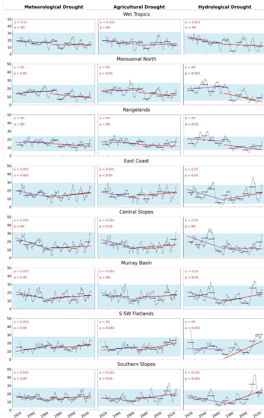
365 Figure 4: 5 year rolling mean of area under drought for the three traditional drought metrics over the NRM areas. The trend from 1911-1965 is shown in magenta, and the trend from 1966-2020 in red. The significance of these trends are indicated in the top left hand corner of each plot ( p = \text{N/S} : not significant, p < 0.05 : significant, p < 0.001 : very significant). The black horizontal bars represent decadal means, and the light blue shading indicates the range of the decadal confidence intervals (Eq. 3).
