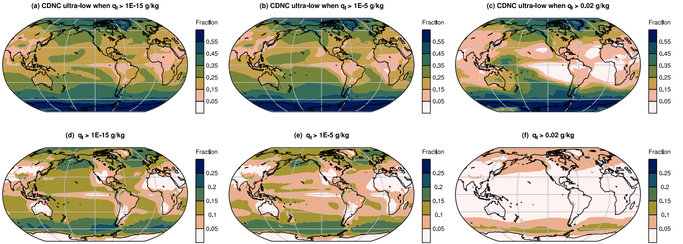
Figure 5. The upper row shows the 10-year mean annually averaged fraction of cloudy time steps and model layers that exhibit ultra-low CDNCs, i.e., the conditional probability P(\text{CDNC ultra-low} | \bar{q}_l \geq q_{l,\min}) . The lower row shows the 10-year mean annually averaged fraction of all model time steps and model layers that are considered “cloudy” because the grid box mean cloud liquid mass mixing ratio of stratiform and shallow convective clouds, \bar{q}_l , is higher than a threshold q_{l,\min} , i.e., the probability P(\bar{q}_l \geq q_{l,\min}) . The three columns correspond to three different choices of q_{l,\min} used in conditional sampling: q_{l,\min} = 10^{-15} \text{ g kg}^{-1} in the left column, q_{l,\min} = 10^{-5} \text{ g kg}^{-1} in the middle column, and q_{l,\min} = 0.02 \text{ g kg}^{-1} in the right column. The fractions (probabilities) were diagnosed in the 10-year free-running nc00 simulation explained in Table 1, i.e., EAMv2 with no lower bound for CDNC. Geographical distribution of the joint probability P(\text{CDNC ultra-low} \cap \bar{q}_l \geq q_{l,\min}) can be found in Fig. S4 in the Supplement. Further details and discussions can be found in Sect. 4.2 .
