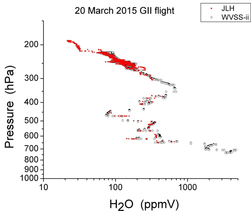
Figure 12. Water vapor profiles from JLH Mark2 and the FLYHT WVSS-II sensor on March 20, 2015, during a NGSC FTB flight.
