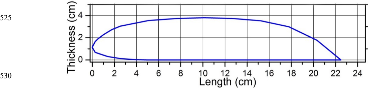
Figure 6. Airfoil shape for zero coefficient of pressure on much of the lower surface.
