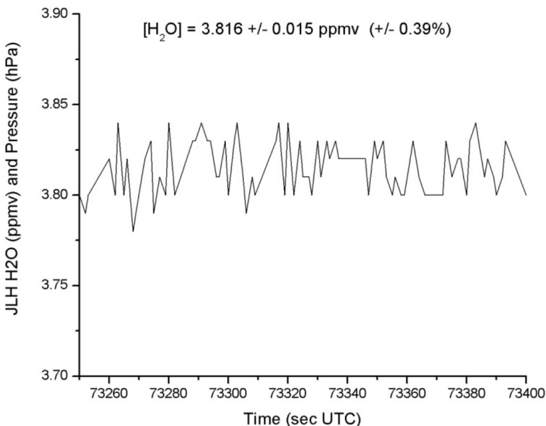
Figure 11. Stratospheric water measurements during level flight of the NASA ER-2 aircraft on 8 Aug 2013 recorded by JLH Mark2. In this flight segment, water vapor is expected to be nearly constant. The standard deviation of the measurement is 0.015 ppmV.
