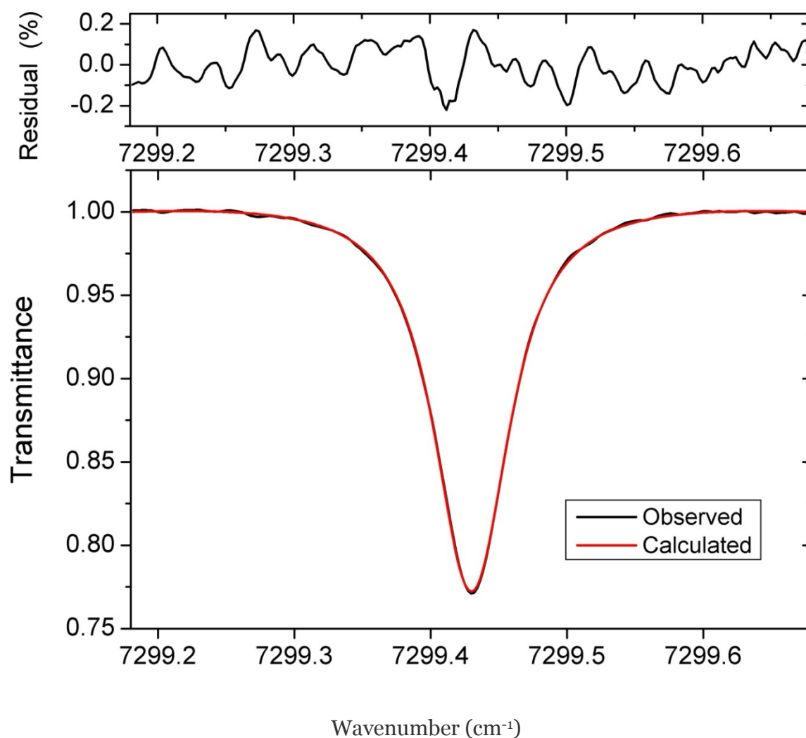
Figure 9. A high ambient pressure transmission spectrum during a flight on Sept 2, 2013, at a pressure of 225.95 hPa (169.48 Torr) and a temperature of 225.19 K. Also shown is a fitted spectrum, yielding a water concentration of 296 parts-per-million by volume (ppmV).
