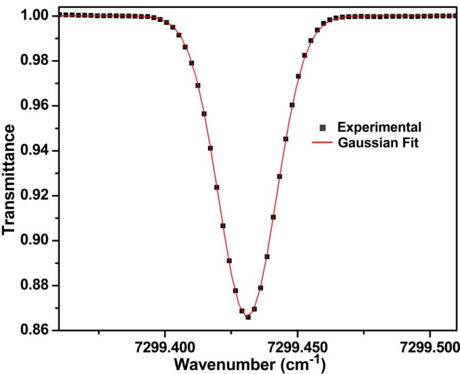
Figure 7. Experimental transmittance spectrum and a Gaussian fit to the data, where the transmittance = 1- absorptance.
