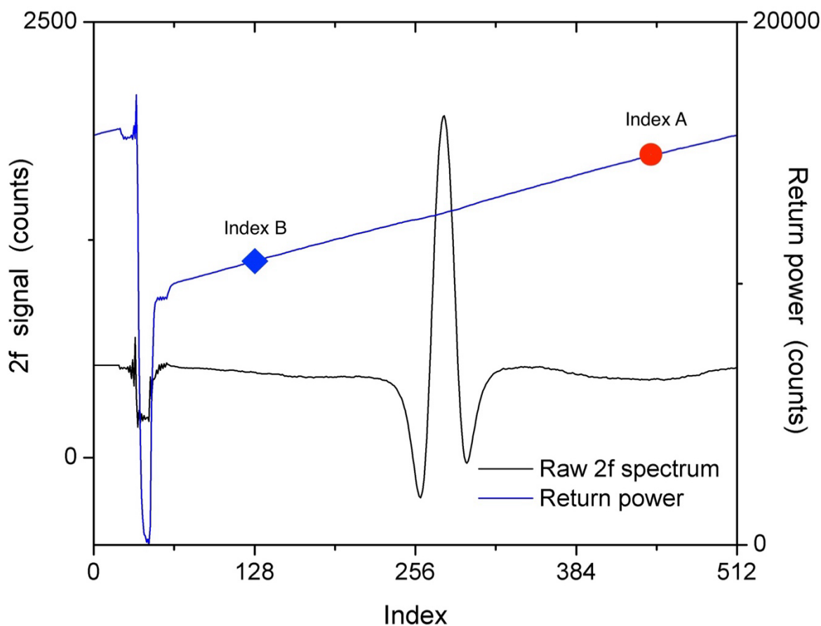
Figure 8. An example second harmonic (2f) spectrum (black trace) and return laser power spectrum (blue trace) acquired with JLH Mark2 during the NASA ER-2 aircraft flight of 2 September 2013. The spectrum was recorded at 82178 sec UTC at a pressure of 129.96 hPa, temperature of 203.3 K and a calculated water volume mixing ratio of 6.81 ppmV. As reference for Figure 10, the return laser power is identified at two points, the blue diamond is Index B and the red circle is Index A.
