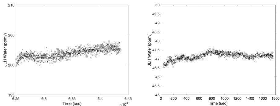
Figure 5. Time series of JLH water vapor measurement inside the laboratory calibration chamber with continuous flow of air/water vapor mixture from the TS3900 humidity generator. (a) Left plot is 200 ppmV input at 57.2 hPa total pressure and 295.4 K temperature, (b) Right plot is 50 ppmV input at 120.3 hPa total pressure and 296.4 K temperature.
