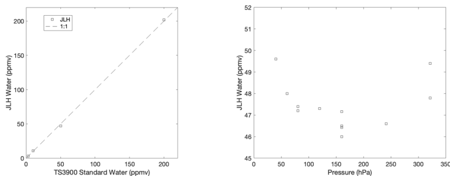
395 Figure 5. (c) Left plot shows the relation of JLH water measurement to TS3900 water source. A 1:1 line (dashed line) is also shown. (d) Right plot is JLH water measurement inside lab calibration chamber at different total pressures while the TS3900 provides a constant source of 50 ppmV water vapor at room temperature.
