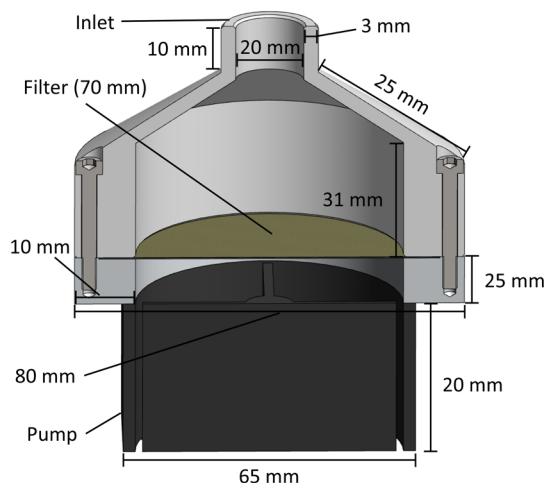
85 Figure 1: Schematic representation of the filter holder. The air containing aerosol particles is sucked through the filter, which is positioned on a stainless-steel mesh.
