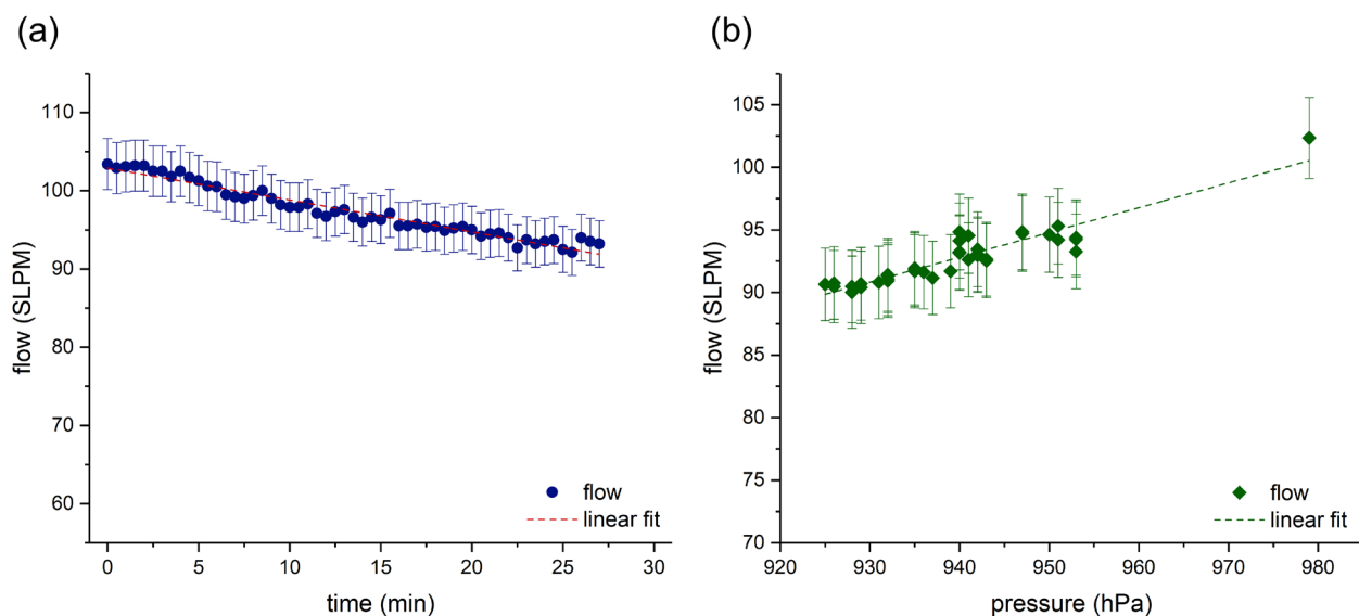
Figure 2: (a) Flow through the filter holder as a function of time (at 980 hPa) (blue dots), the dashed line represents a linear fit of the data. The errors correspond to 2% of the measured value, which represents the measurement uncertainty of the flow meter (b) Flow through the filter holder as a function of pressure (green diamonds), the dashed line represents a linear fit of the data. The errors correspond to 2% of the measured value, which represents the measurement uncertainty of the flow meter.
