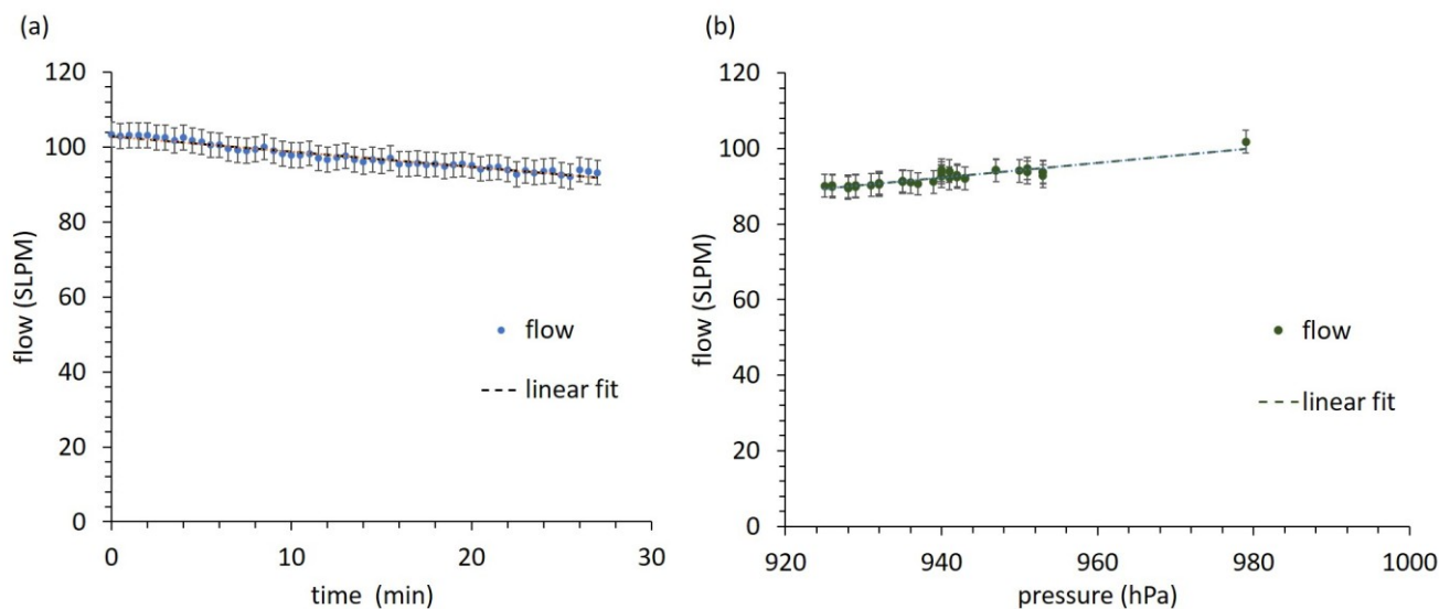
Figure 2: (a) shows the flow through the filter holder as a function of time (at 980 hPa) (blue dots), the dashed line represents a linear fit of the data. The errors correspond to 2% of the measured value, which represents the measurement uncertainty of the flow meter. (b) shows the flow through the filter holder as a function of pressure (green dots), the dashed line represents a linear fit of the data. The errors correspond to 2% of the measured value, which represents the measurement uncertainty of the flow meter. 135
