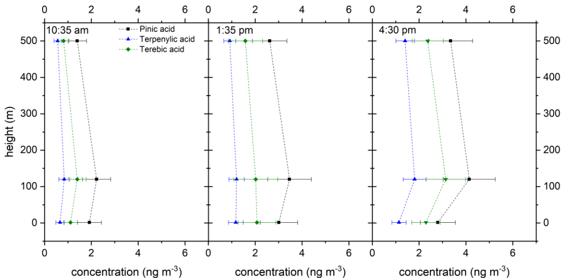
195 Figure 5: Vertical profiles of the biogenic marker compounds pinic acid (black square), terpenylic acid (blue triangle) and terebic acid (green diamond) at the different times (all times are in UTC+2). For better clarity, these points are connected by dashed lines The error bar is the result of two error sources: the standard deviation derived from the triple determination made by the LC-MS measurement; and the error associated with the flow measurement of the filter holder.
