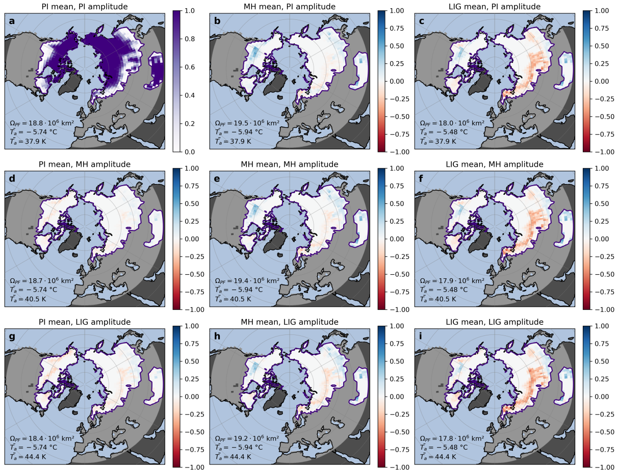
Figure 4. Simulated permafrost probabilities ( p_{FF} ) for all climate forcings, shown as absolute values for the PI experiment in panel a, and as anomalies for all other experiments. The results for the original climate forcings are shown on the diagonal (PI: a; MH: e; LIG: i), and the off-diagonal panels show results for the alternative climate forcings, with each column having the same mean temperature (PI: a,d,g; MH: b,e,h; LIG: c,f,i) and each row having the same seasonal temperature amplitudes (PI: a,b,c; MH: d,e,f; LIG: g,h,i). The purple line marks the limits of the joint permafrost domain of all simulations. The permafrost area ( \Omega_{PF} ), the mean annual temperature ( \bar{T}_a ), and the mean seasonal temperature amplitude ( \bar{T}_a ) for the joint permafrost domain are given in the lower left corner of each panel.
