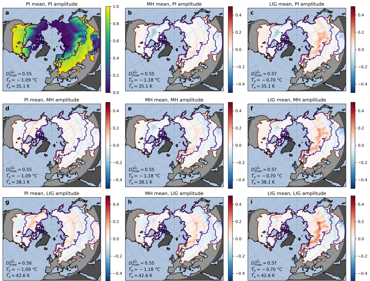
Figure A2. Same as Fig. A1, but for the annual thawed ground fraction ( D_{thaw}^{3m} ). The mean annual thawed ground fraction ( D_{thaw}^{3m} ), the mean annual temperature ( \bar{T}_a ), and the mean temperature amplitude ( \tilde{T}_a ) for the joint seasonal frost domain are given in the lower left corner of each panel.
