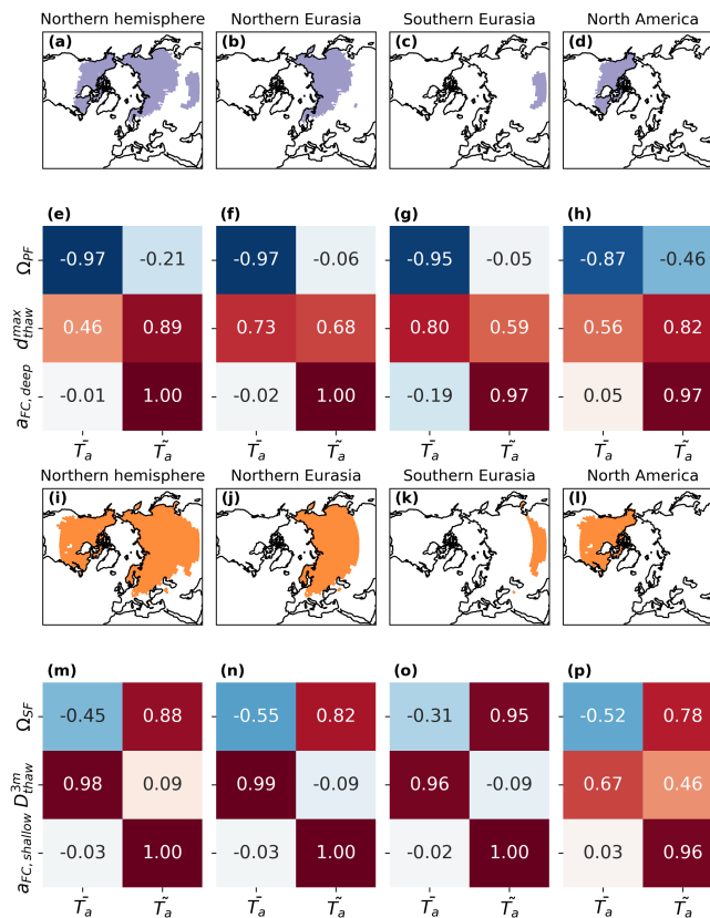
Figure 5. Northern hemisphere and regional Pearson correlations between different diagnostics and the mean temperatures ( \bar{T}_a ) and the seasonal temperature amplitudes ( \bar{T}_a ) of all nine experiments. Panels a-d and i-l respectively show the part of the joint permafrost and seasonal frost domains which are considered for the correlation analysis in the panels below (northern hemisphere: lat>30°N; northern Eurasia: lat>40°N, 0°E<lon<186°E; southern Eurasia: lat<40°N, 0°E<lon<186°E; North America: lat>30°N, 186°E<lon<360°E). For the joint permafrost domain (e-h), we considered the permafrost area ( \Omega_{PF} ), the maximum thaw depth ( d_{thaw}^{max} ), and the deep thermal contraction cracking activity ( a_{FC,deep} ). For the joint seasonal frost domain (m-p), we considered the seasonal frost area ( \Omega_{SF} ), the thawed ground fraction ( D_{thaw}^{3m} ), and the shallow thermal contraction cracking activity ( a_{FC,shallow} ).
