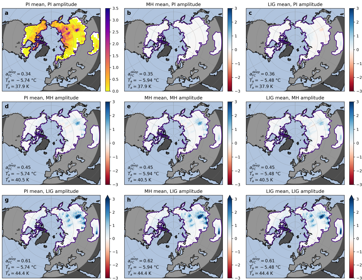
Figure 7. Same as Fig. 4, but for the deep thermal contraction cracking activity ( a_{FC}^{deep} ). The mean deep thermal contraction cracking activity ( a_{FC}^{deep} ), the mean annual temperature ( \bar{T}_a ), and the mean seasonal temperature amplitude ( \bar{T}_a ) for the joint permafrost domain are given in the lower left corner of each panel.
