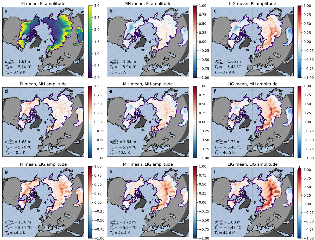
Figure 6. Same as Fig. 4, but for the simulated maximum thaw depths ( d_{thaw}^{max} ). The mean maximum thaw depth ( d_{thaw}^{max} ), the mean annual temperature ( \bar{T}_a ), and the mean seasonal temperature amplitude ( \tilde{T}_a ) for the joint permafrost domain are given in the lower left corner of each panel.
