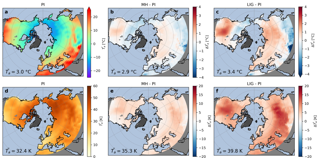
Figure 1. Overview of the mean ( \bar{T}_a ) and seasonal amplitude ( \bar{\Delta T}_a ) of surface temperatures in the simulation domain. Absolute values are shown for the PI (a,d), and anomalies relative to the PI are shown for the MH (b,e) and the LIG (c,f).
