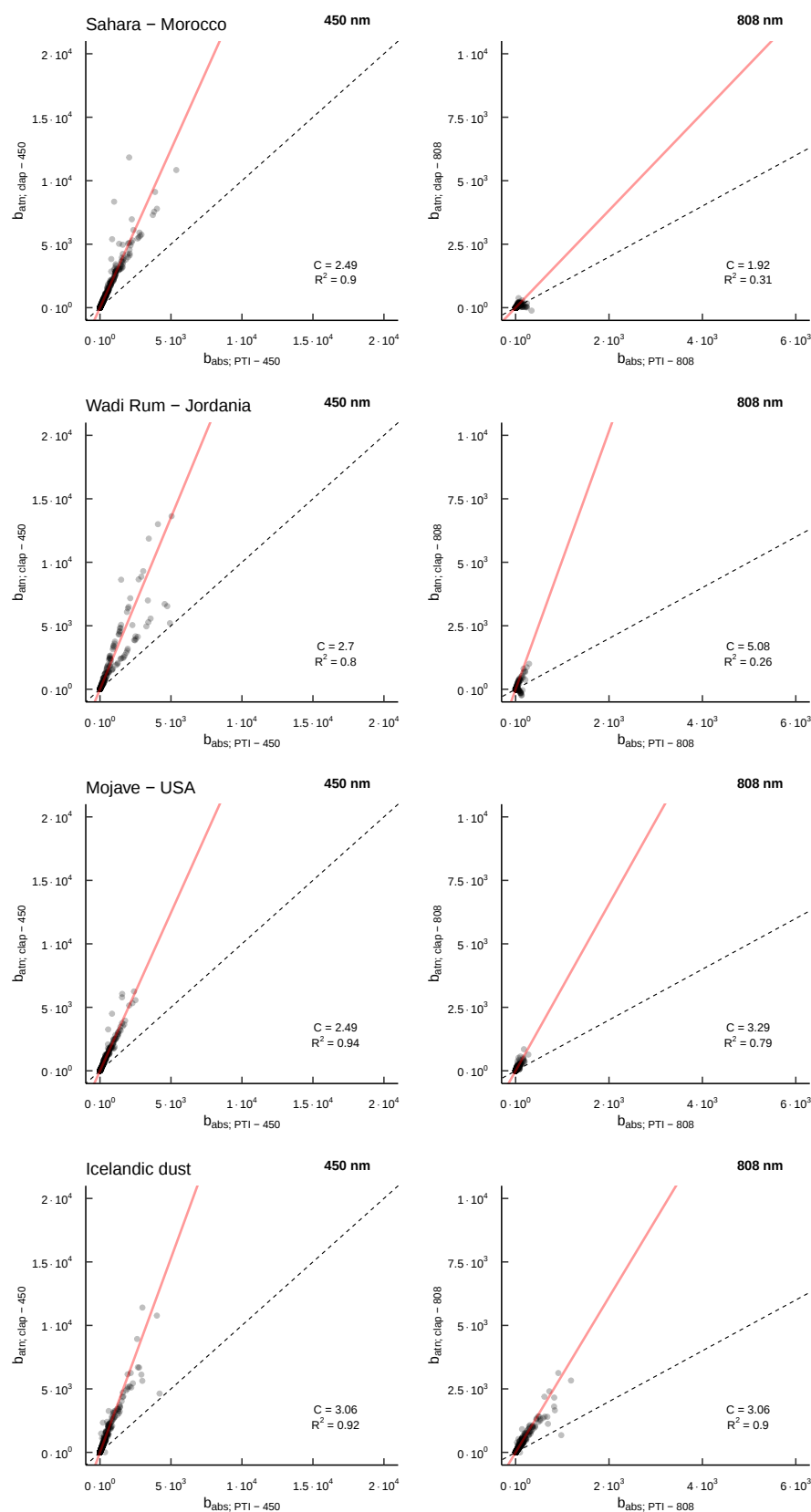
Figure S18: CLAP attenuation corrected for the scattering artefact vs the PTAAM-2 \lambda absorption coefficient at 450 (left panels) and 808 nm (right panels) for the mineral dust samples analysed during the laboratory experiments. In particular, each panel is for the regions: a) Saharan mineral from Morocco, b) dust from Wadi Rum, c) Mojave desert (USA) and d) Icelandic dust. The slope represents the multiple scattering parameter C .
