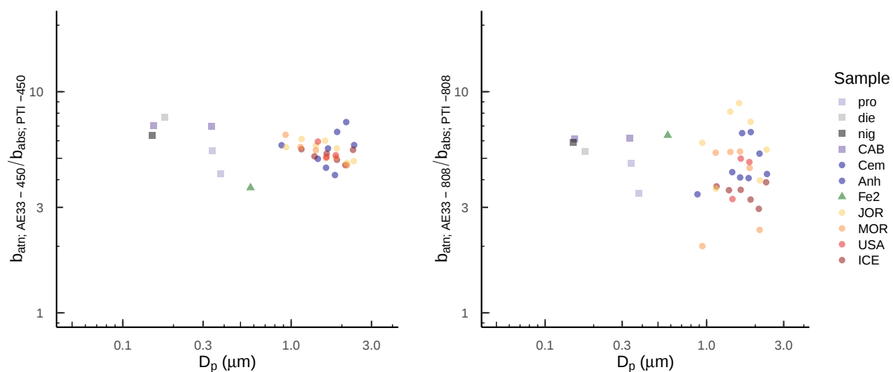
Figure S25: Multiple scattering parameter C , for AE33 and CLAP FPs vs the volume particle diameter for each of the sample groups analyzed during the laboratory measurements. It was obtained as the ratio of the FP's attenuation corrected for the scattering artefact and the PTAAM- 2\lambda absorption coefficient at 450 and 808 nm.
