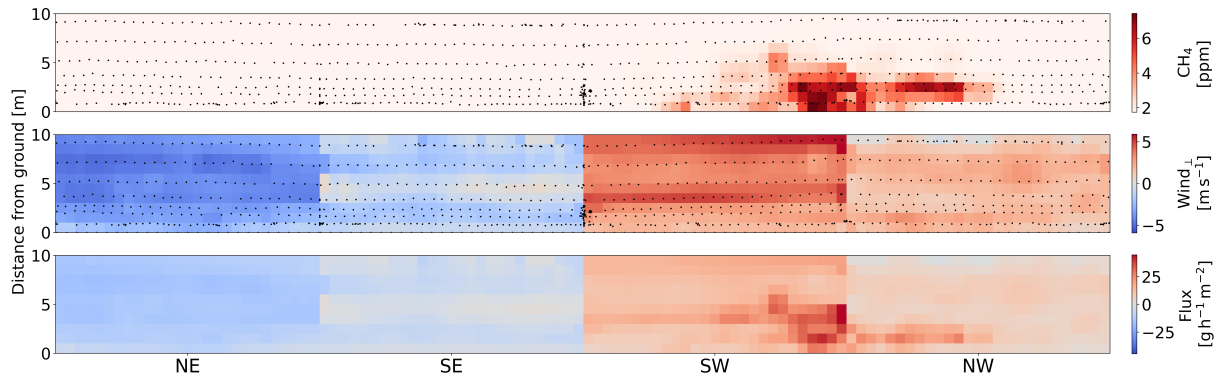
Figure 4. Results of the mass balance approach for a drone flight in the afternoon of 6 March 2024 with a herd of 208 heifers. The panels show (top) the interpolated CH 4 concentration observations, (middle) the interpolated perpendicular wind speeds, and (bottom) the CH 4 fluxes across the vertical sampling planes. Positive (negative) perpendicular wind speeds and fluxes correspond to flow out of (into) the box. The black scatter points indicate the original observation locations.
