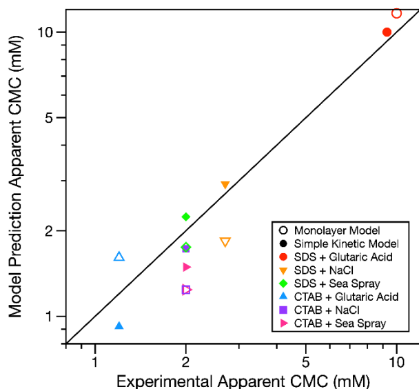
Figure 2: Comparison of the apparent CMC predictions for 6 \mu\text{m} radius droplets from the Simple Kinetic and Monolayer Models to the experimentally determined apparent CMCs. The black 1:1 line indicates where model predictions and experimental observations are identical. Error bars have been omitted for clarity, but uncertainty in the CMC is generally within 10%.
