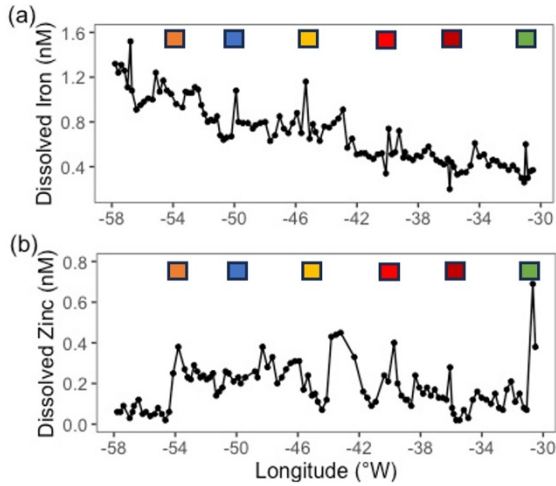
310 Figure 2. Zonal gradients in (a) dissolved iron concentrations (nM, from Kunde et al., 2019) and (b) dissolved zinc concentrations (nM). Samples captured from the towed FISH at \sim 7\text{m} . Coloured square represent stations sampled during JC150 (see Fig. 1 for station names).
