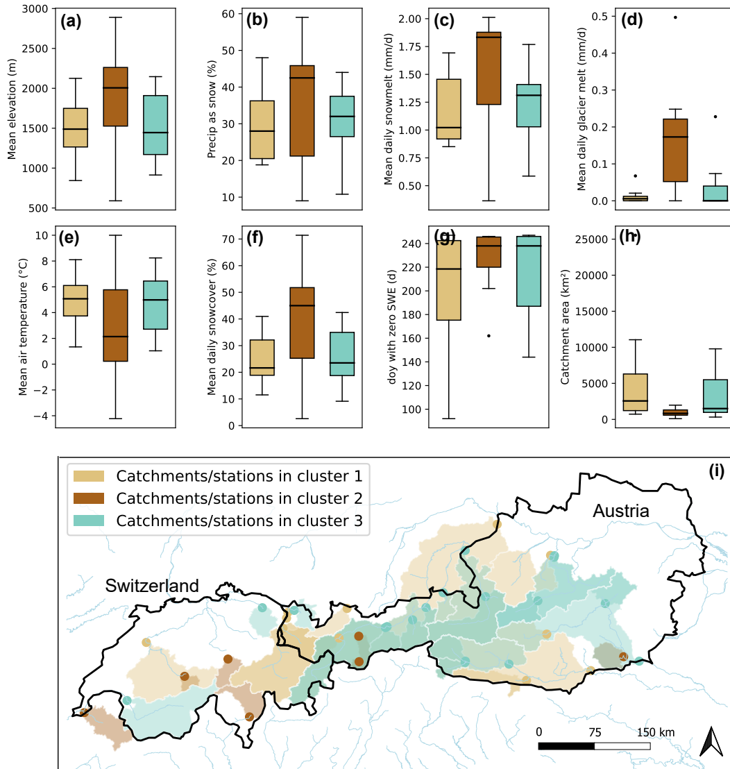
Figure 4. Panels (a-h) illustrate eight catchment characteristics and their distribution across the three different clusters and within each cluster (the internal distribution is visualised by the boxplots). Panel (i) maps the spatial location of the (nested) catchments over Switzerland and Austria.
