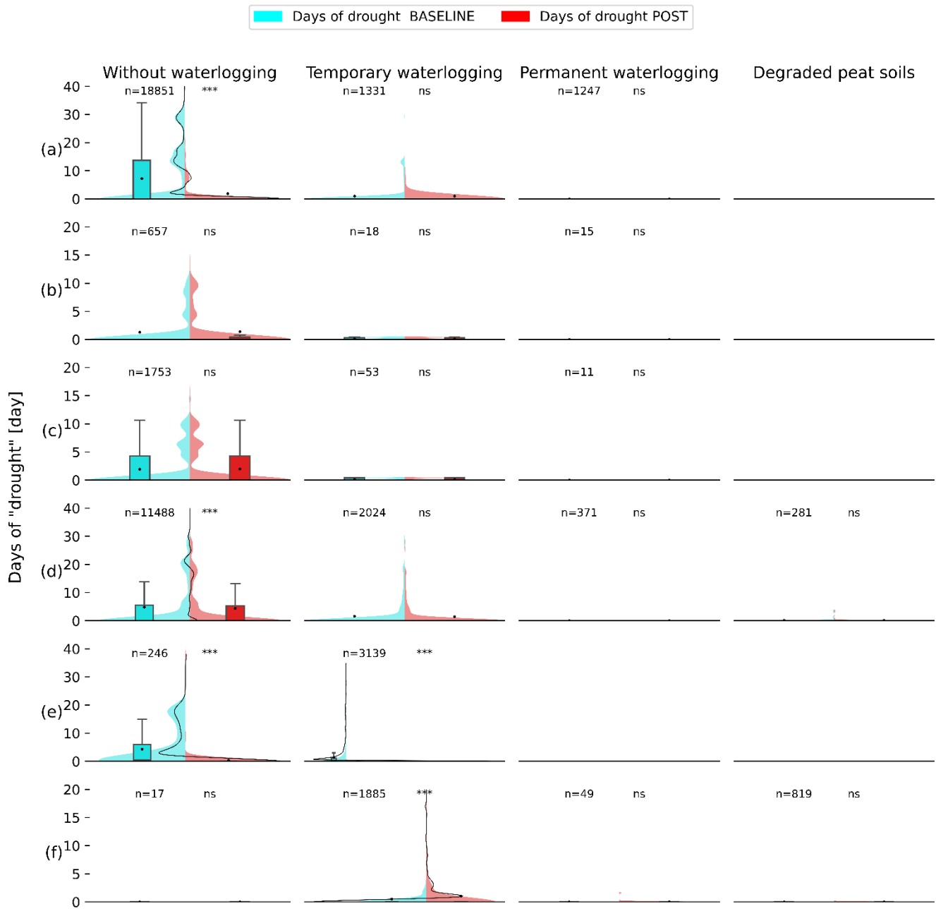
Figure 9: Comparison of days of drought (matrix potential of -30m and return period of 25 years) before (BASELINE) and after (POST) implementing NbS (a : Hedgerows, b : Reduced tillage, c : Soil pitting, d : Forest practices aimed at limiting soil compaction, e : Forest diversification with practices aimed at limiting soil compaction, f : Restoration of peatlands) for each drainage classification from the Belgian soil map. Each data points (n) represent the infiltration of one model grid cell. Significance levels - ns (p-value>0.05), * (0.01<p-value<0.05), ** (0.001<p-value<0.01), *** (p-value<0.001) - indicate results of Kolmogorov-Smirnov tests comparing BASELINE and POST distributions. The centred vertical black lines depict the difference in kernel density estimates between different BASELINE and POST distributions.
