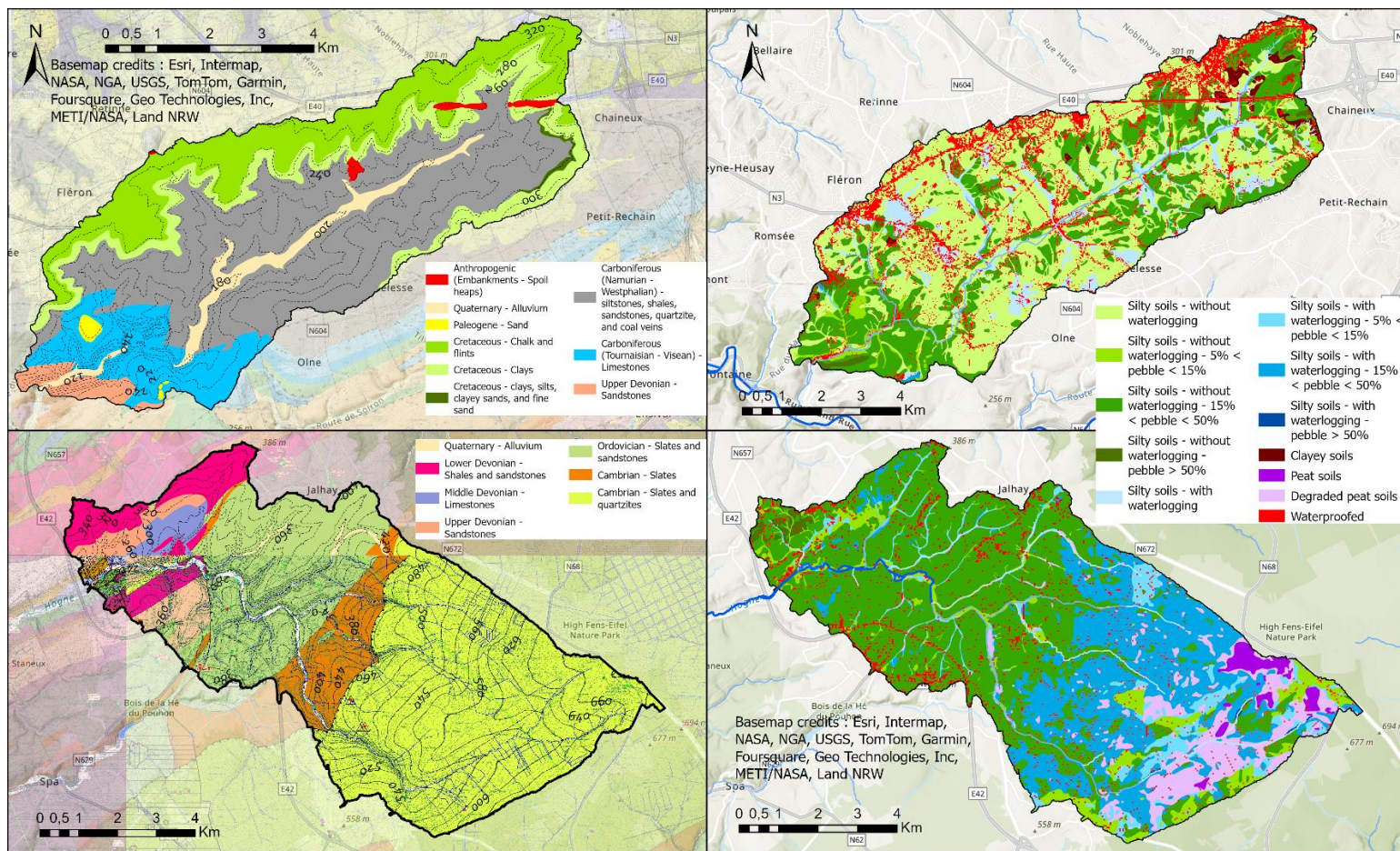
185 Figure 2 : (Geological maps of C1 and C2, showing the absolute age of geological units (Period, Epoch, or Age) and the principal rock types within these units (Carte Géologique de Wallonie, 2025; Carte hydrogéologique de Wallonie, 2025). Soil maps of C1 and C2, depicting textural classes, natural drainage characteristics, and stoniness (Carte Numérique des Sols de Wallonie, 2023).
