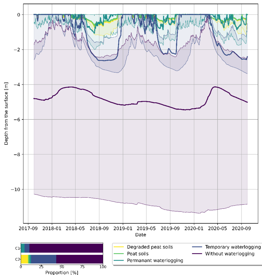
Figure 4: Modelled saturated zone depth (watersheds C1 and C2) based on drainage classes from the Belgian soil map. The thick line represents the median values calculated from each model cells for each drainage class. The thin lines indicate the 25th and 75th percentiles. The stacked bar chart represents the relative proportion of surface of natural drainage classes of soils found in C1 and C2.
