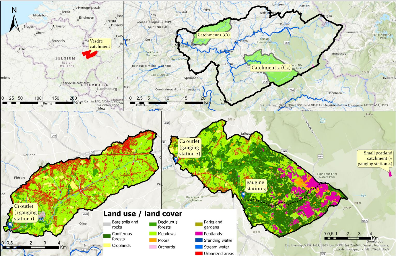
145 Figure 1: Study area with maps of land use/ land cover and soils.
