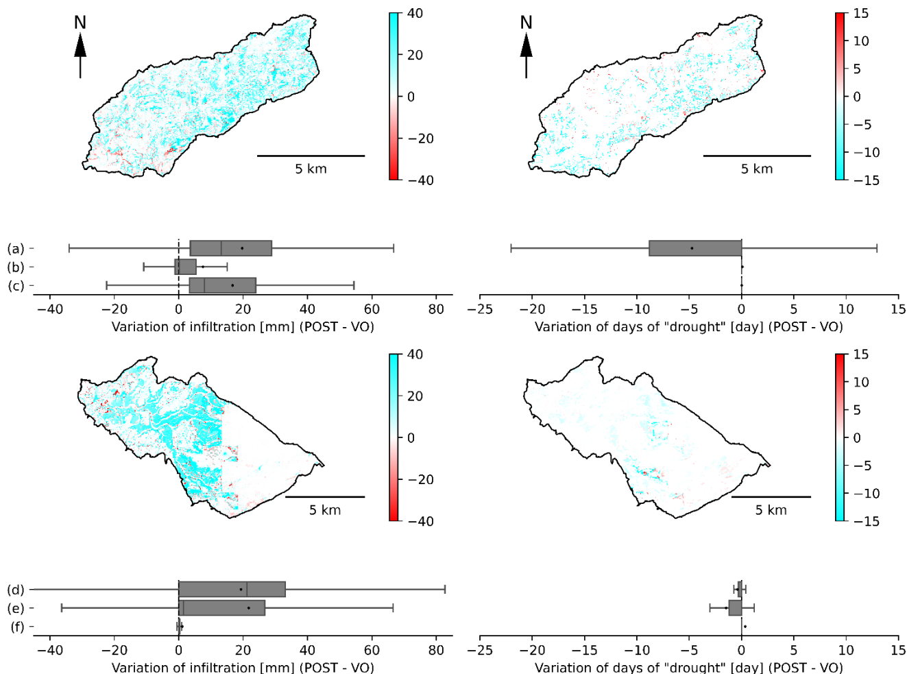
Figure 6: Variation of cumulative infiltration (from 13 to 18 July 2021) and days-of-drought of Vegetation Drought Stress Duration (matric potential of -30m and return period of 25 years) on model grid cells before (BASELINE) and after (POST) implementing NbS (a : Hedgerows, b : Reduced tillage, c : Soil pitting, d : Forest practices aimed at limiting soil compaction, e : Forest diversification with practices aimed at limiting soil compaction, f : Restoration of peatlands).
