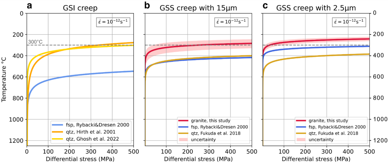
Figure 9: Comparison of deformation mechanisms of quartz (qtz), feldspar (fsp) and granite at common viscous strain rates of 10^{-12}\text{s}^{-1} . (a) is GSI creep, where quartz is the weakest rheology, (b) and (c) show GSS creep with 15 and 2.5 \mu\text{m} , where fsp and granite become weaker than quartz GSS with 15 \mu\text{m} and even weaker than quartz GSI creep at 2.5 \mu\text{m} . The 300°C line across all plots points at the observed onset of GSS creep in nature. References as in Fig. 9.
