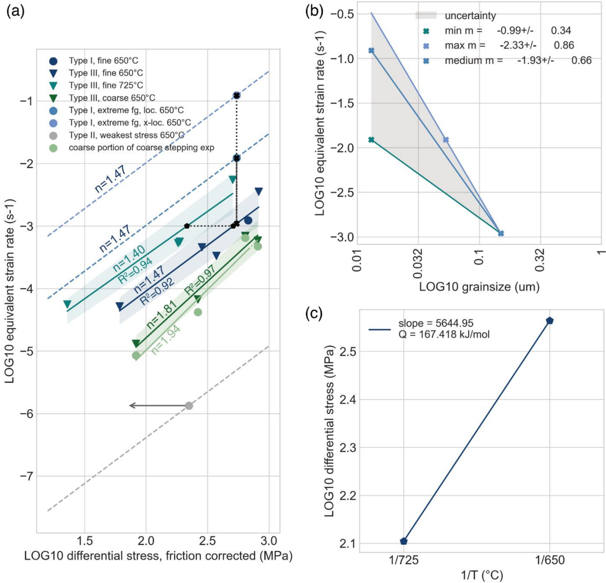
Figure 6: Calculations of rate, grain size and temperature dependencies for interpretations and extrapolations. (a) n -value calculations based on mostly Type III experiments taken from steady state/highest strain value . Assumptions and extrapolations see text. Arrow in grey indicates that this Type II experiment did not reach steady state stress yet and therefore might continue to weaken. Furthermore, its strain rate is a minimum value, however, localization might mean strain rates to up to 10^{-4} s -1 . (b) Minimum and maximum grain size dependency taken at the points marked with a cross in (a). (c) Temperature dependence/activation energy calculations based on the pentagon points in (a), taking into account several experiments and experimental data points. Verification of calculated parameters in Supplementary.
