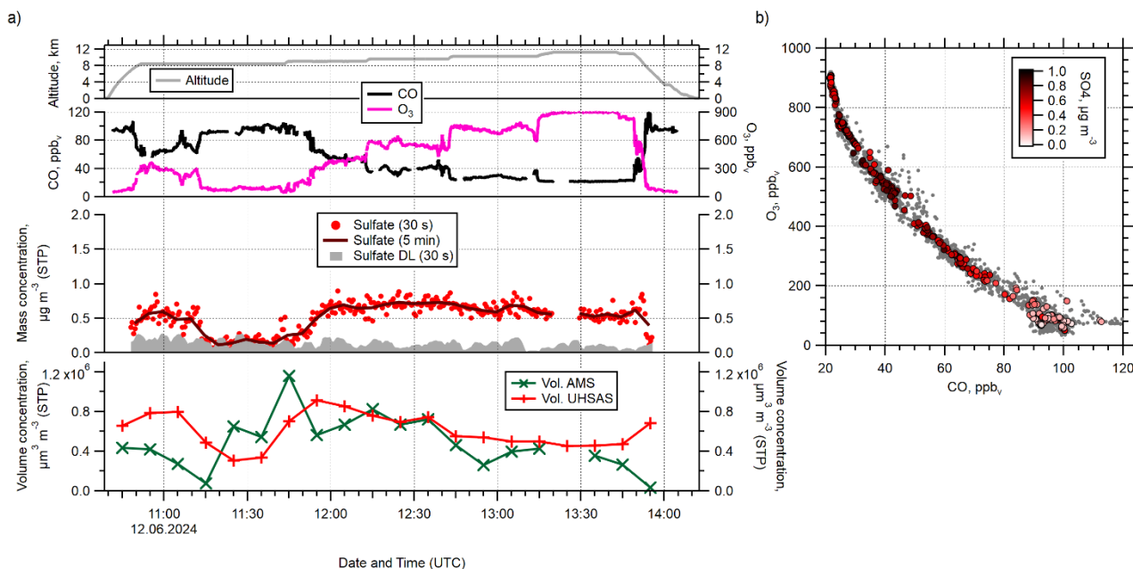
500 Figure 11: (a) Time series of O_3 , CO , and particulate sulfate from research flight 4 of the TPEX campaign (June 12, 2024). Shown are the raw data (30 s), a 5-min average, and the detection limit for the 30 s resolution. The lowest panel shows a comparison between the total volume concentration measured by the CARIBIC-AMS and a UHSAS operated in parallel on the Learjet. (b) Tracer-tracer plot with O_3 and CO , color-coded by sulfate mass concentration.
