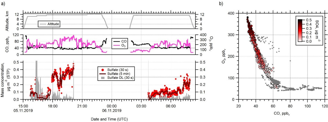
Figure 10: (a) Time series of O 3 , CO, and particulate sulfate from IAGOS-CARIBIC flights FL578 and FL579, conducted on November 05 and 06, 2019, between Munich and Boston. (b) Tracer-tracer plot with O 3 and CO, color-coded by sulfate mass concentration.
