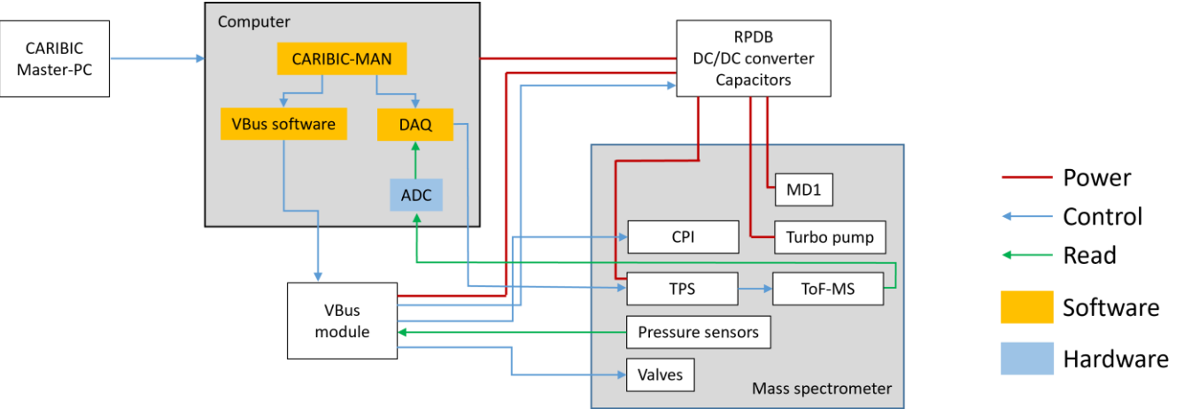
Figure A1: Schematic representation of the software and hardware hierarchy of the CARIBIC-AMS: The main control software running on the computer is CARIBIC-MAN, while the VBus software is controlling the VBus module which in turn controls the hardware components such as the RPDB (Rack Power Distribution Box), the valves and the CPI. CARIBIC-MAN also controls the data acquisition software (DAQ) that controls the ToF power supply (TPS) and reads the data through the analog-digital converter (ADC).
