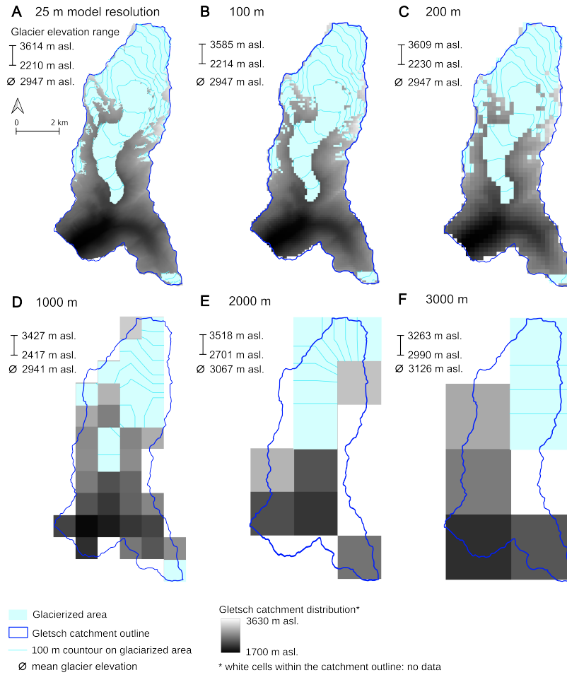
Figure 3. Glacier and catchment representation across various model resolutions. The resolution is given at the top of each panel and ranges between 25 m and 3000 m. Light blue represents the glacierized area, characterized by the light blue contour lines. For each case, the original (high-resolution) catchment outlines are drawn in blue for reference.
