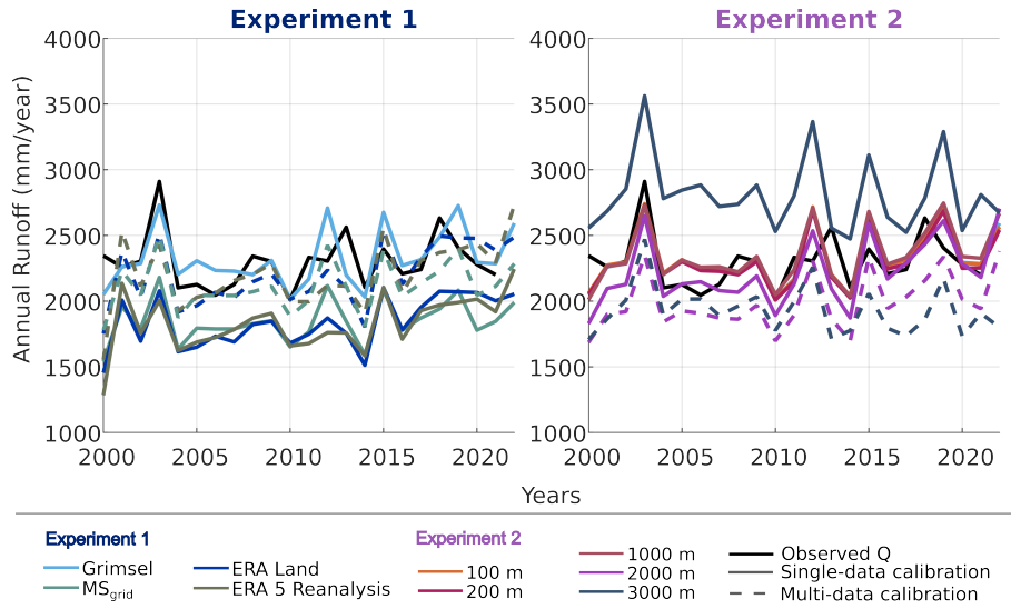
Figure 8. Annual catchment runoff observed and simulated using different (A) forcing products and (B) model resolutions. Simulations calibrated with a single parameter (solid lines) and with a two-parameter (dashed lines) calibration scheme are distinguished. For model resolutions <2000 m, the annual runoff results are independent of the calibration method.
