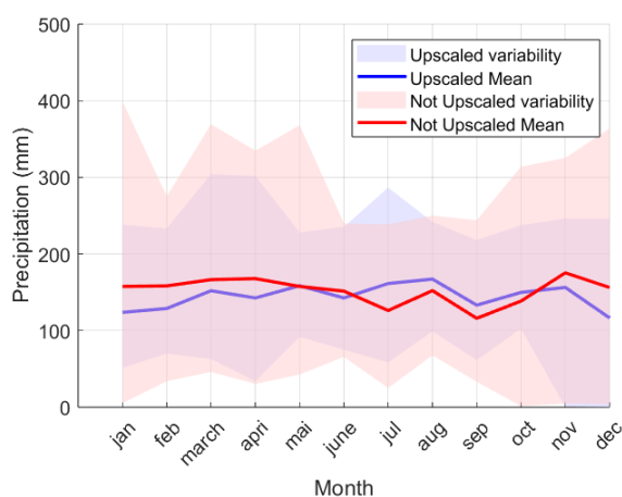
Figure S2: Comparison between the mean 2000-2022 precipitation from the MS_{grid} product for both the upscaled (blueish) and not upscaled (reddish) methods. Colored area shows the variability of precipitation, while the line corresponds to the mean precipitation.
