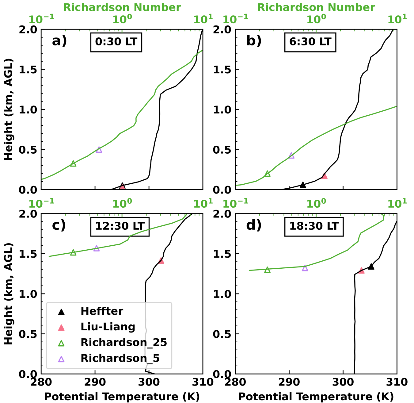
Figure 1. PBLHT estimates from the PBLHT-SONDE VAP during the four SONDE launches on May 8, 2017. Since PBLHTs from Heffter and Liu-Liang methods primarily rely on potential temperature profiles, their PBLHT estimates are plotted alongside these profiles. PBLHTs from the bulk Richardson method are plotted on the corresponding Ri profiles. Richardson_25 refers to PBLHT estimate using a Ri_c threshold of 0.25, while Richardson_5 refers to a Ri_c threshold of 0.5. AGL stands for Above Ground Level, and all altitudes in this study are in terms of AGL.
