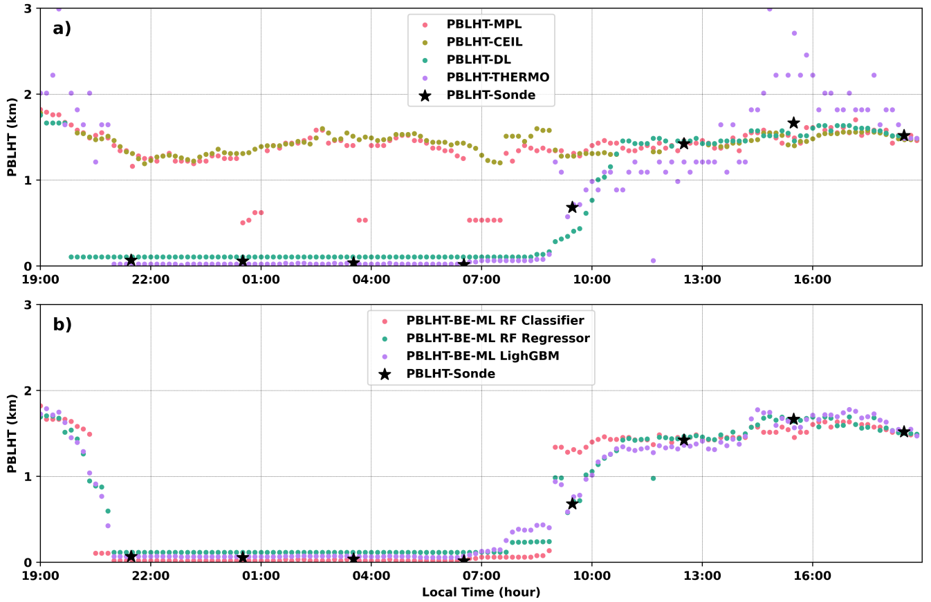
Figure 9. PBLHT estimates on July 12, 2019, at the ARM SGP site: a) PBLHT estimates from individual remote sensing measurements and PBLHT-Sonde; b) PBLHT-BE-ML prediction from the three ML models and PBLHT-Sonde.
