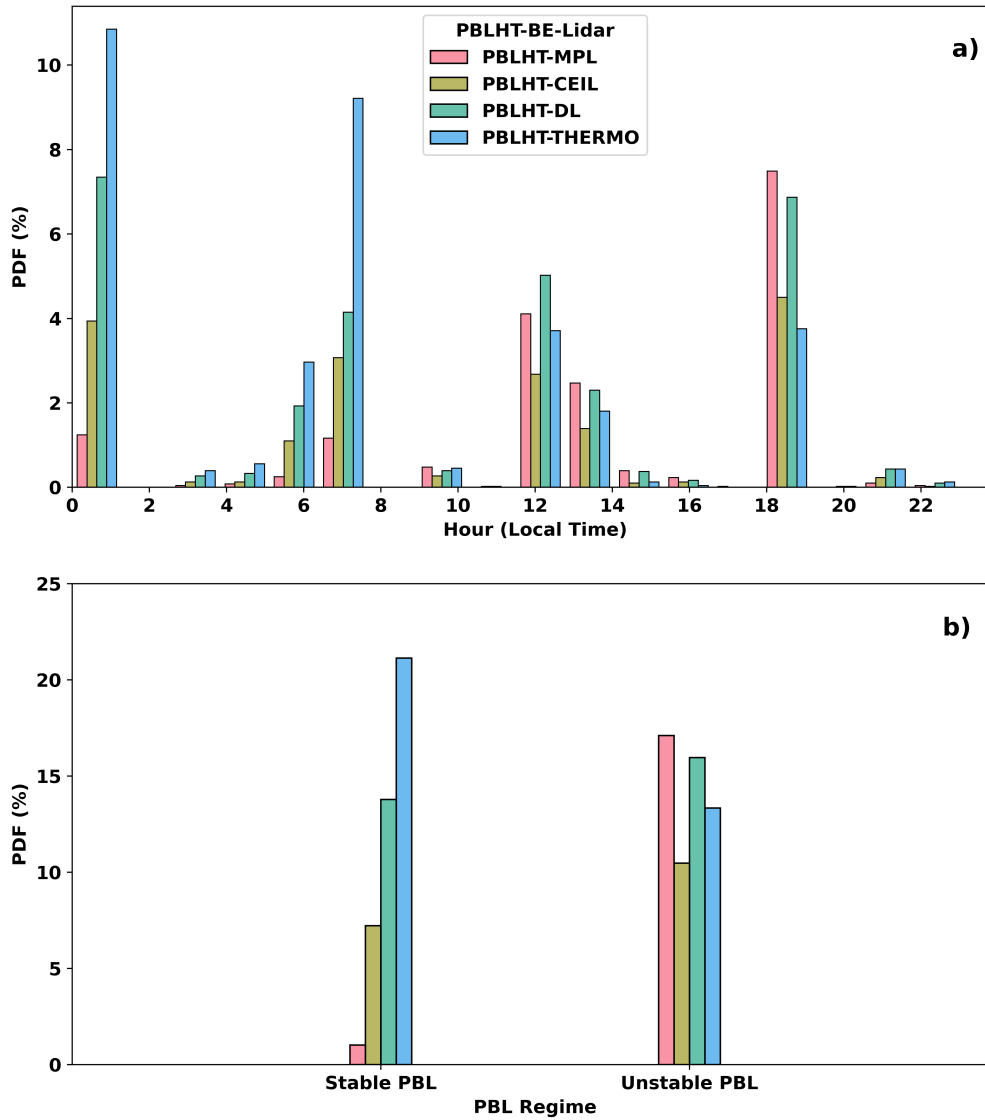
Figure 6. Histogram plots of probability distribution functions (PDFs) of PBLHT estimates from remote sensing measurements that are selected as the PBLHT-BE-Lidar at different LTs (a) and PBL regimes (b).
