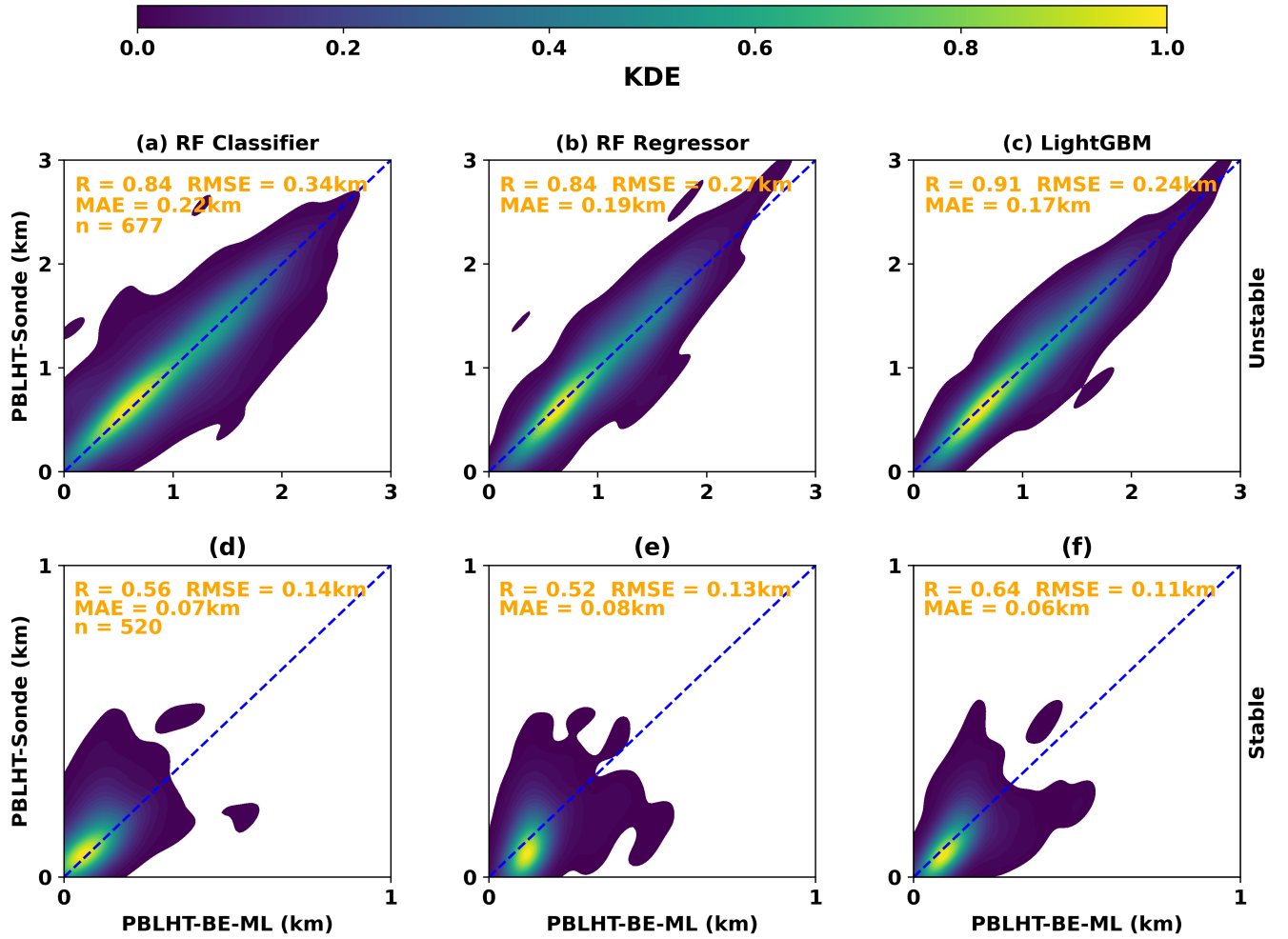
415 Figure 7. Similar as Figure 4, but for comparisons of predicted PBLHT-BE-ML from ML methods with PBLHT-Sonde.
