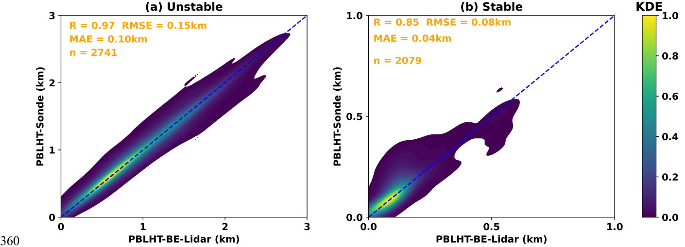
360 Figure 5. Similar as Figure 4., but for comparisons of PBLHT-BE-Lidar and PBLHT-Sonde.
