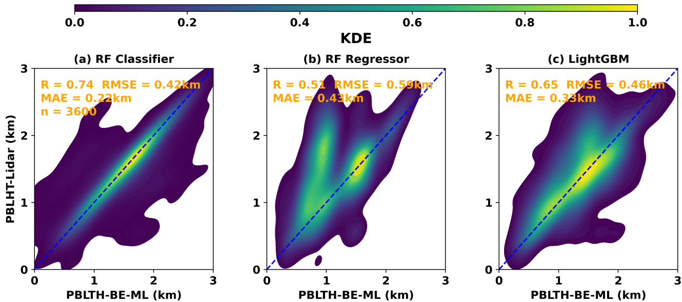
530 Figure 11. Similar as Figure 4, except for comparisons of predicted PBLHT-BE-ML against PBLHT-Lidar from: a) RF Classifier; b) RF Regressor; c) LightGBM under afternoon convective PBL conditions between 14:00 and 18:00 local time during summer and fall at the ARM SGP site.
