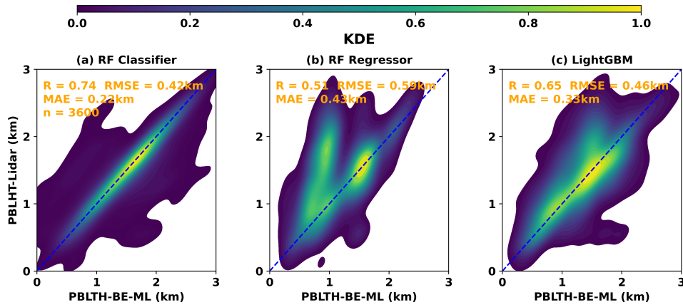
550 Figure 11. Similar as Figure 4, except for comparisons of predicted PBLHT-BE-ML against PBLHT-Lidar from: a) RF Classifier; b) RF Regressor; c) LightGBM under afternoon convective PBL conditions between 14:00 and 18:00 local time during summer and fall at the ARM SGP site.
