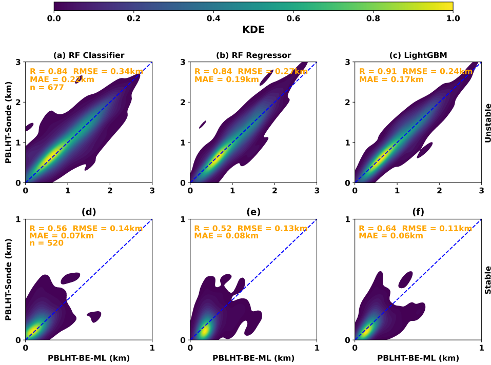
425 Figure 7. Similar as Figure 4, but for comparisons of predicted PBLHT-BE-ML from ML methods with PBLHT-Sonde.
