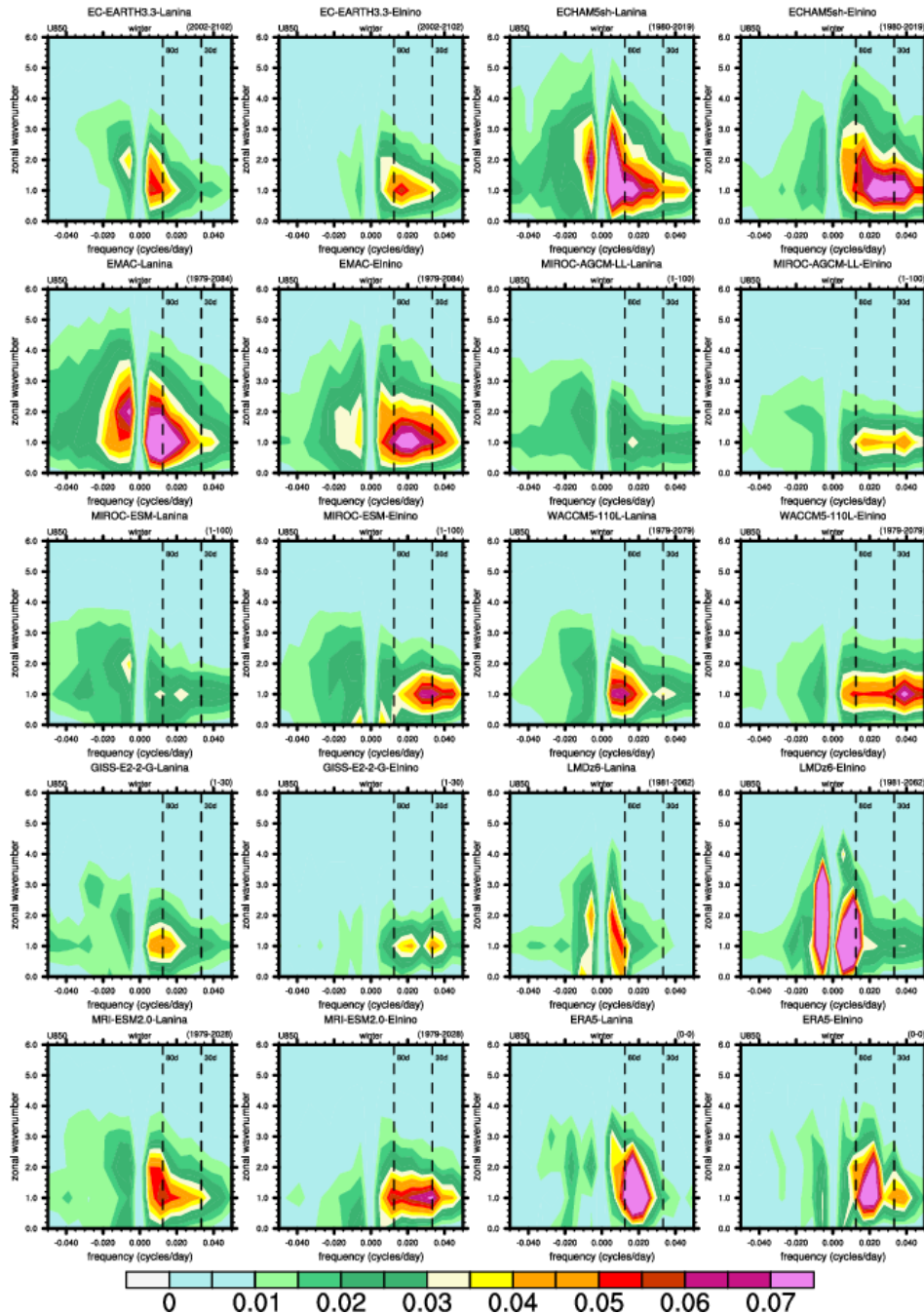
Figure 3: November-April wavenumber-frequency power spectra of 10°S–10°N averaged U850. Units of the U850 spectrum are \text{m}^2/\text{s}^2 per frequency interval per wavenumber interval. We interpret the power at \sim 180 -day frequencies as a by-product of using centered November-April segments.
