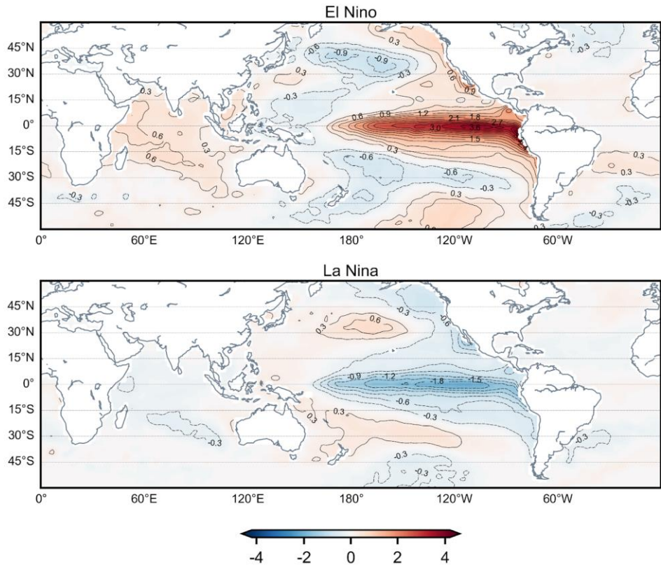
Figure 1: November-April composites of the El Niño (top) and La Niña (bottom) JMA COBE SST anomalies (units K) that are prescribed in the perpetual ENSO simulations.
