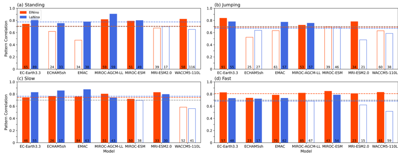
Figure 5: Pattern correlations between the ERA5 and simulated time-longitude (Hovmöller) 10°S-10°N convective OLR anomaly composites ( OLR < -5 \text{ W/m}^2 ) corresponding to each of the four k-means clusters MJO archetypes defined in Wang et al. (2019). Multi-model average El Niño and La Niña correlations are shown by red and blue dashed lines, respectively. The gray dashed line marked at a correlation of 0.7 is a heuristic threshold (Back et al. 2024) to decide when a particular model’s MJO archetype is well captured by a model and bars are shaded in red or blue when correlation exceeds this threshold. Number of events is printed at the bottom of each bar.
