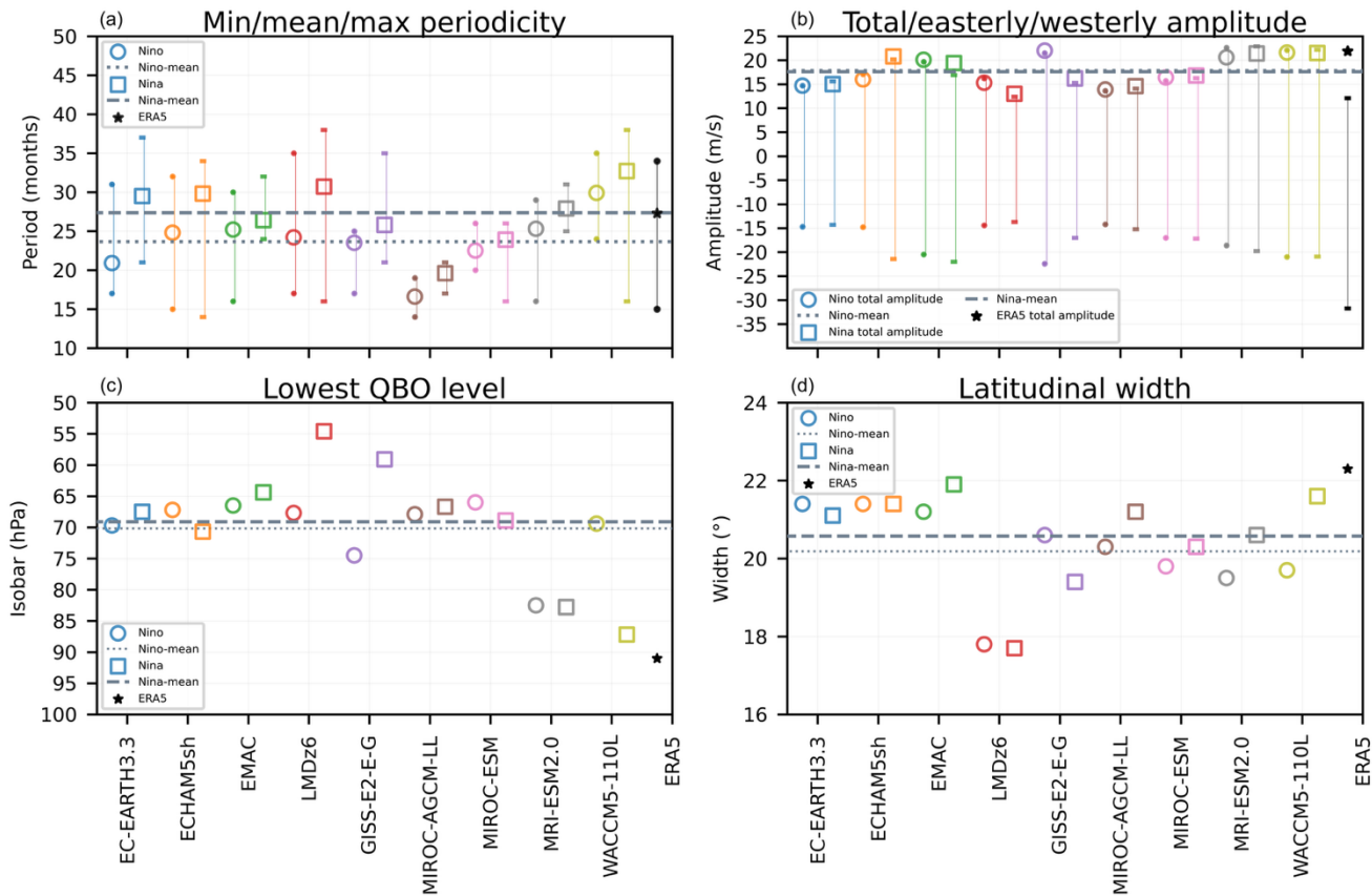
537 538 Figure 7: Periodicity, amplitude, lowest level of descent, and latitudinal width of the QBO in El Niño (circles) and La Niña (squares) 539 simulations. (a) mean periodicity, where whiskers extend to the minimum and maximum period, El Niño mean is dotted, La Niña 540 mean is dashed, and ERA5 is shown in black. (b) circles and squares show total amplitudes (“TT amplitude” from Richter et al. 541 2020), tops of whiskers show westerly amplitudes, and bottoms of whiskers show easterly amplitudes. (c) lowest isobar the QBO 542 descends to, the level at which the QBO Fourier amplitude falls to 10% of its maximum. (d) latitudinal width of QBO, full width at 543 half amplitude maximum of a Gaussian fit to the QBO Fourier amplitude
