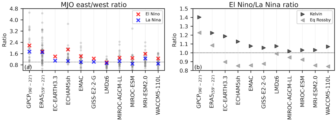
Figure 4: (a) Ratio of eastward to westward MJO precipitation spectral power (from Figure 2) filtered for wavenumbers +/- 1 to 3 and 30 to 96 day frequencies. Red and blue X's denote El Niño and La Niña, respectively, using the same notation for both the GPCP and ERA5 composite averages and the climatological values from the perpetual El Niño and La Niña simulations. Gray dots indicate interannual east/west ratios from GPCP, ERA5, and the QBOi Experiment 1 simulations (1979-2009 AMIP) by these same models; EC-EARTH3.3 and GISS-E2-2G did not run Experiment 1. (b) Ratio of Kelvin wave and equatorial Rossby wave power in El Niño to that in La Niña. Each wave is filtered using equivalent depths of 8 to 90 meters, with wavenumbers of 1 to 14 for the Kelvin wave and -1 to -10 for the equatorial Rossby wave.
