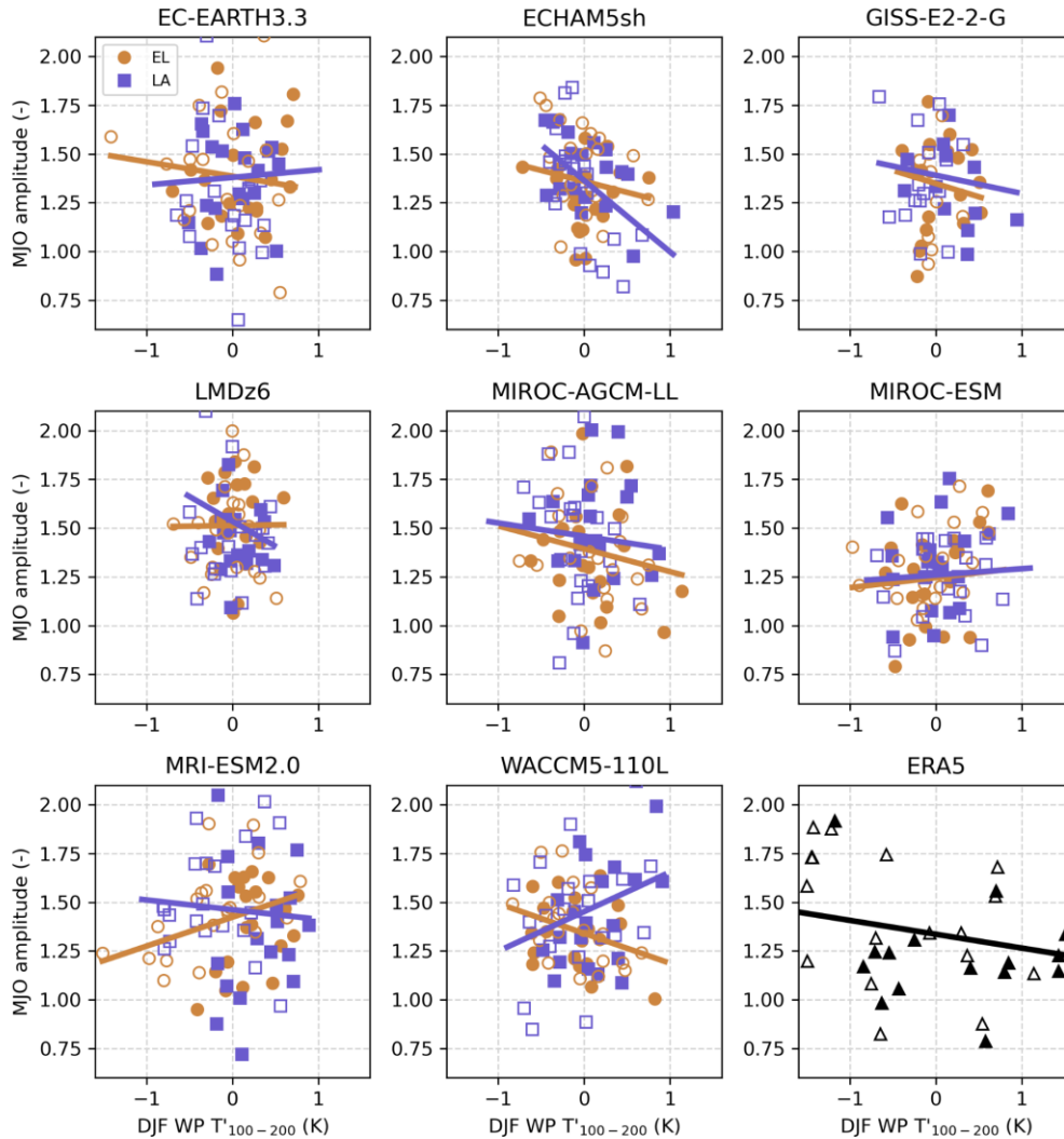
Figure 8: Scatter plot of warm-pool averaged ( 10^{\circ}\text{S} - 10^{\circ}\text{N} , 45^{\circ}\text{E} - 180^{\circ}\text{E} ) tropopause stability anomalies (100 hPa minus 200 hPa temperature) versus December-February MJO amplitude. Lines represent the slope of the regression line during El Niño (orange) or La Niña (purple). Easterly and westerly QBO phases, which are delineated by the sign of the December-February 5^{\circ}\text{S} - 5^{\circ}\text{N} 50 hPa zonal mean zonal-wind, are denoted by open and filled markers, respectively.
