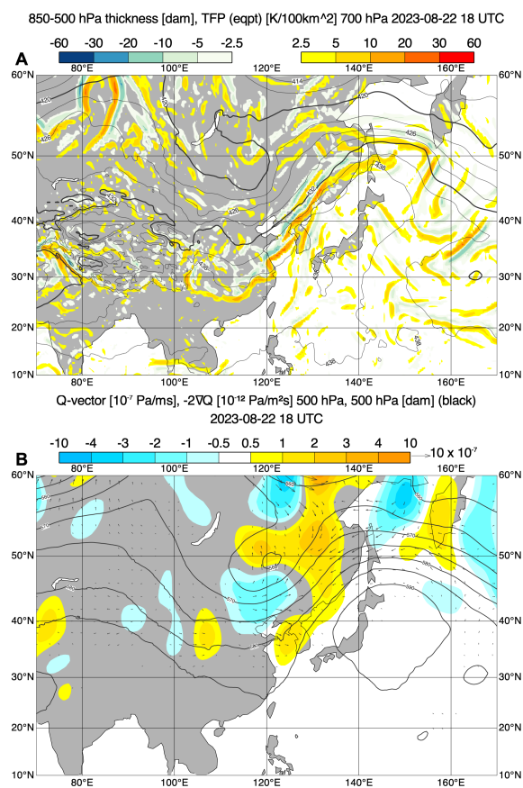
Figure 10. Analyse maps from 2023-08-22 18 UTC. A shows the thermal front parameter (TFP) and 850–500 hPa thickness. B shows Q-Vector, Q-Vector vergences, and 500 hPa geopotential.
