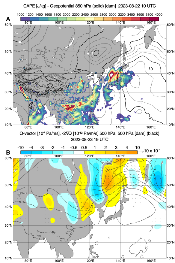
Figure 9. Analyse map from 2023-08-22 10 UTC ( A ) and 2023-08-23 19 UTC ( B ). A shows the vertical distribution of the Convective Available Potential Energy (CAPE) and 850 hPa geopotential. B shows Q-Vector, Q-Vector vergences, and 500 hPa geopotential.
