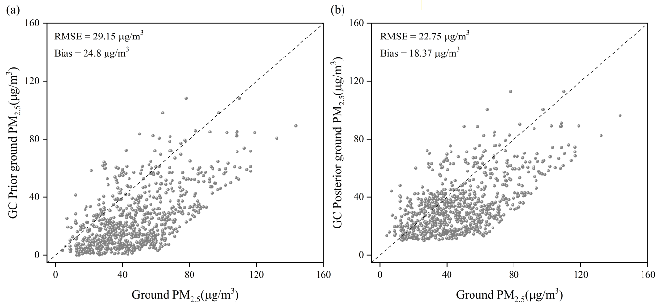
Figure 8. Scatter plot of the ground-observed against the \text{PM}_{2.5} simulation over South Asia either using the prior (a) or using the posterior (b) emission inventory in 2019.
