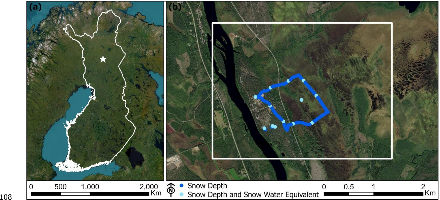
108 109 Figure 1: Study area (a) in Sodankylä, Finland and (b) automated and manual snow depth and snow water equivalent measurements 110 within the 10 km 2 local scale study site. Image credits: © Esri, Earthstar Geographics, and Maxar.
