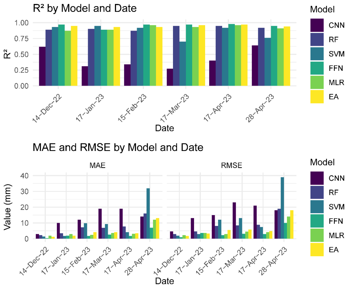
Figure 8: Machine learning model metrics for estimated snow water equivalent with CNN , RF, SVM , FFANN , MLR, and EA. MAE and RMSE are in mm.
