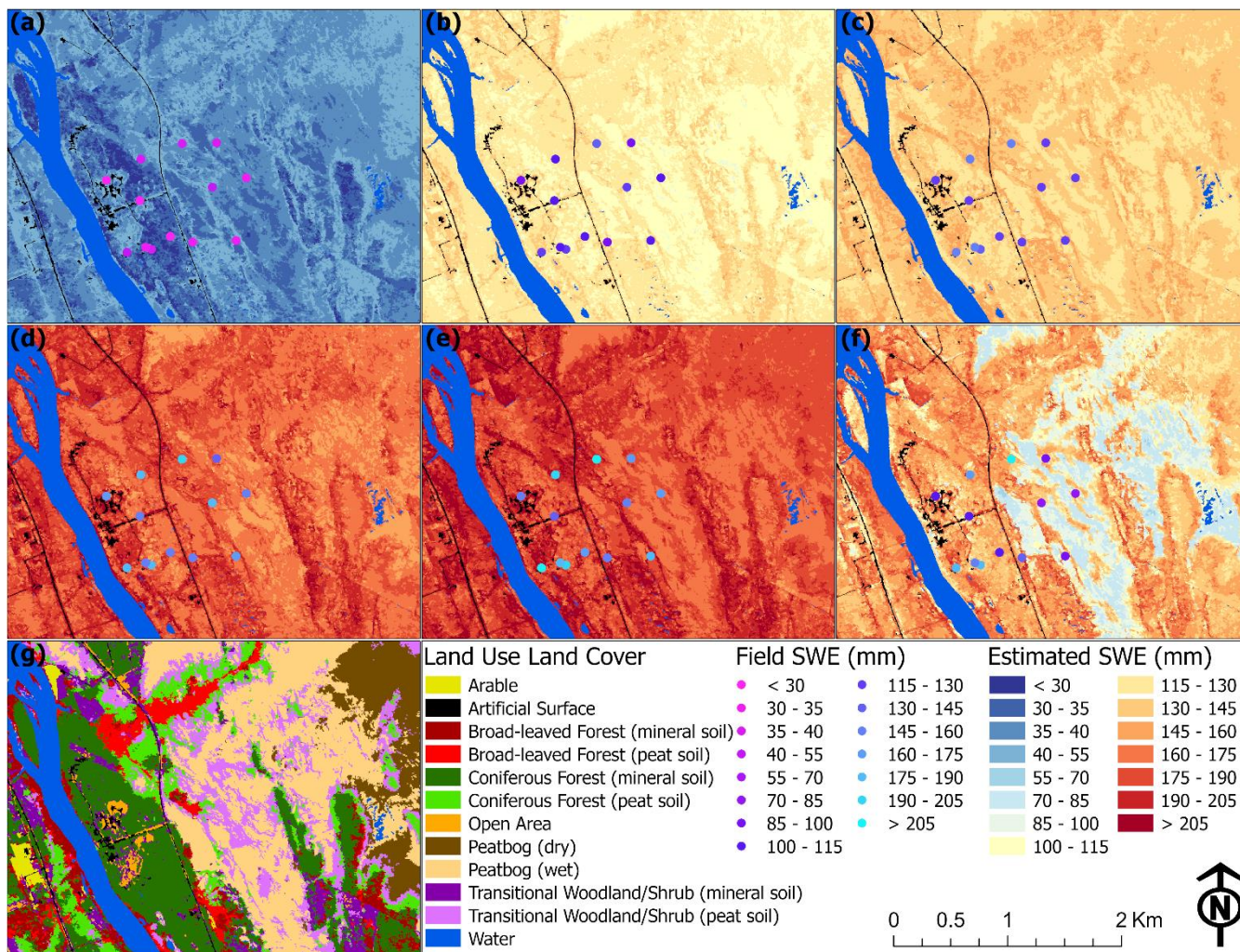
Figure 11: Field and estimated SWE (mm) in a) 14-December-22, b) 17-January-23, c) 15-February-23, d) 17-March-23, e) 17-April-23, and f) 28-April-23 alongside g) a LULC map.
