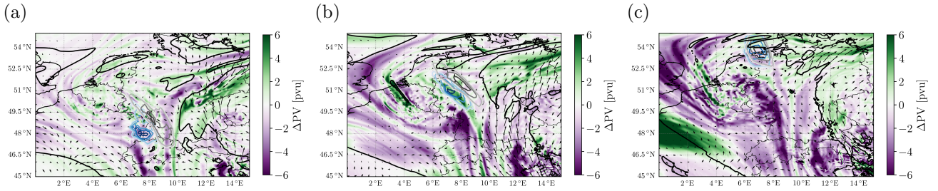
Figure 12. Difference in PV at 10.5 km altitude between the ICON simulations initialized at 12 UTC 06 May 2013 and 00 UTC 07 May 2013. The three panels correspond to valid times (a) 1 UTC, (b) 7 UTC and (c) 13 UTC on 07 May 2013, respectively. The arrows indicate the difference wind field at the same altitude. The contours show the position of back trajectories from the measurement area calculated with the wind field data from the 00 UTC 07 May 2013 (grey) and 12 UTC 06 May 2013 (blue), respectively.
