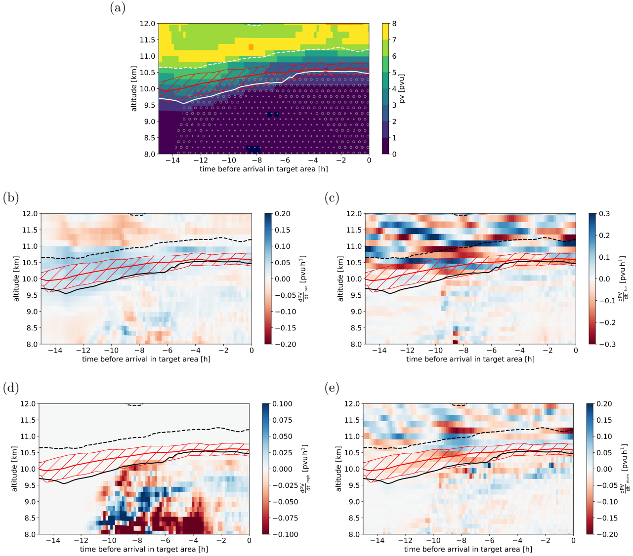
Figure A6. Composite profile along air parcels arriving in the measurement area with pv \geq 2 \text{ p[sv]} and q_i \geq 10^{-3} \text{ mg kg}^{-1} from the simulation started at 12 UTC 06 May 2013: Variables shown are (a) PV, (b) PV tendency from radiation parameterization, (c) PV tendency from latent heating by turbulence parameterization, (c) PV tendency from microphysics parameterization, and (d) PV tendency from momentum transport by turbulence parameterization. The columns have been retrieved from 10 min Eulerian output at the native ICON grid and have been interpolated to the horizontal location of the air parcels.
