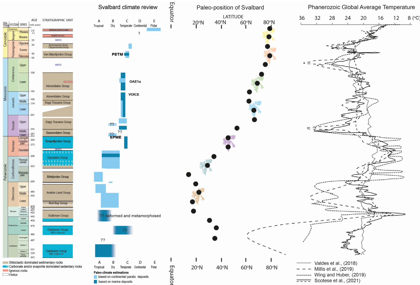
Figure 13. Correlation of the Phanerozoic climate plot based mainly on climate-sensitive facies (See Supplementary material), supplemented by biological and geochemical proxies with the paleogeographic position of Svalbard (Scotese and Wright, 2018) and compilation of the published global average temperature curves.
