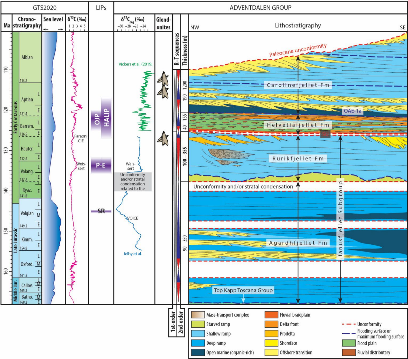
960 Figure 11. Overview of the Upper Jurassic and Lower Cretaceous stratigraphy of Svalbard plotted against time, from Jelby et al. (2024), based on Grundvåg et al. (2017; 2019). To the left of the stratigraphic summary chart, thicknesses of the formations, first- and second-order regressive-transgressive sequences, occurrence of glendonites (Vickers et al., 2019), LIP volcanic episodes (see references in Vickers et al., 2023), and organic stable carbon isotopes (see Jelby et al., 2024 and references therein) are shown. These 965 are plotted against global \delta^{13}\text{C} trends, sea level, and ages from the Geological Time Scale 2020 (Gale et al., 2020; Hesselbo et al., 2020).
