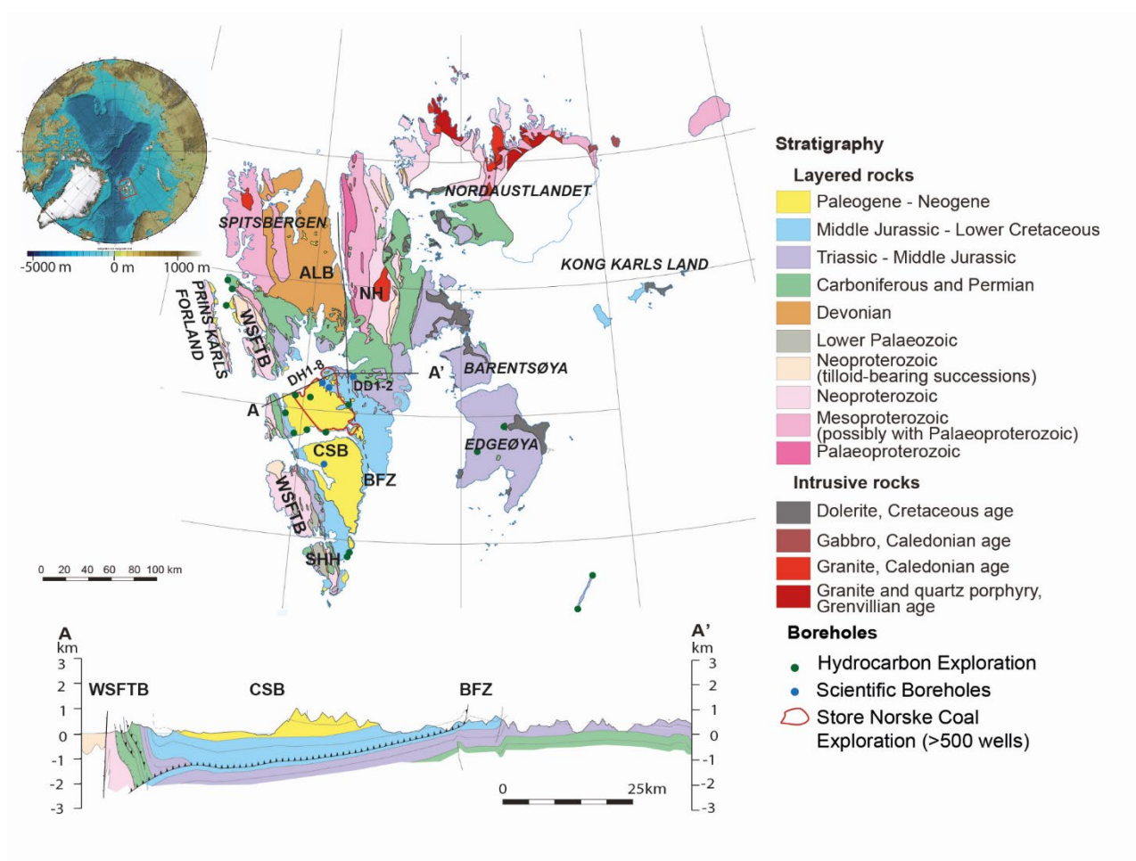
Figure 2: Geological map of Svalbard and a regional cross-section illustrating the major structural elements of central Spitsbergen and spatial coverage of industrial and research boreholes of relevance to deep time paleoclimatic studies. Upper left: International Bathymetric Chart of the Arctic Ocean (IBCAO; Jakobsson et al. (2012)). Geological Map of Svalbard and cross-section (A-A'; bottom) from Dallmann (ed) (2015). Location of boreholes from Senger et al., (2019). NH- Nordfjorden High, SHH- Sørkap Hornsund High, ALB- Andrée Land Basin, BFZ- Billefjorden Fault Zone, WSFTB- West Spitsbergen Fold and Thrust Belt.
