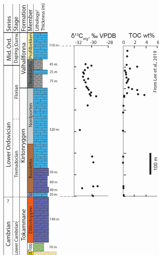
Figure 7 Stratigraphic section of the Cambrian and Ordovician Oslobreen Group succession in Ny Friesland, northern Spitsbergen (see Fig. 5 for location) After Fortey and Bruton (1973); Harland (1997); Stouge et al. (2012); Lehnert et al. (2013); Lee et al., (2019). Bulk organic carbon isotopes ( \delta^{13}\text{C}_{\text{org}} , in ‰ VPDB); Total Organic Carbon (TOC, in weight percent); Bl.- Blårevbreen Member; Topp.- Topiggane Member; Sp.- Spora Member.
