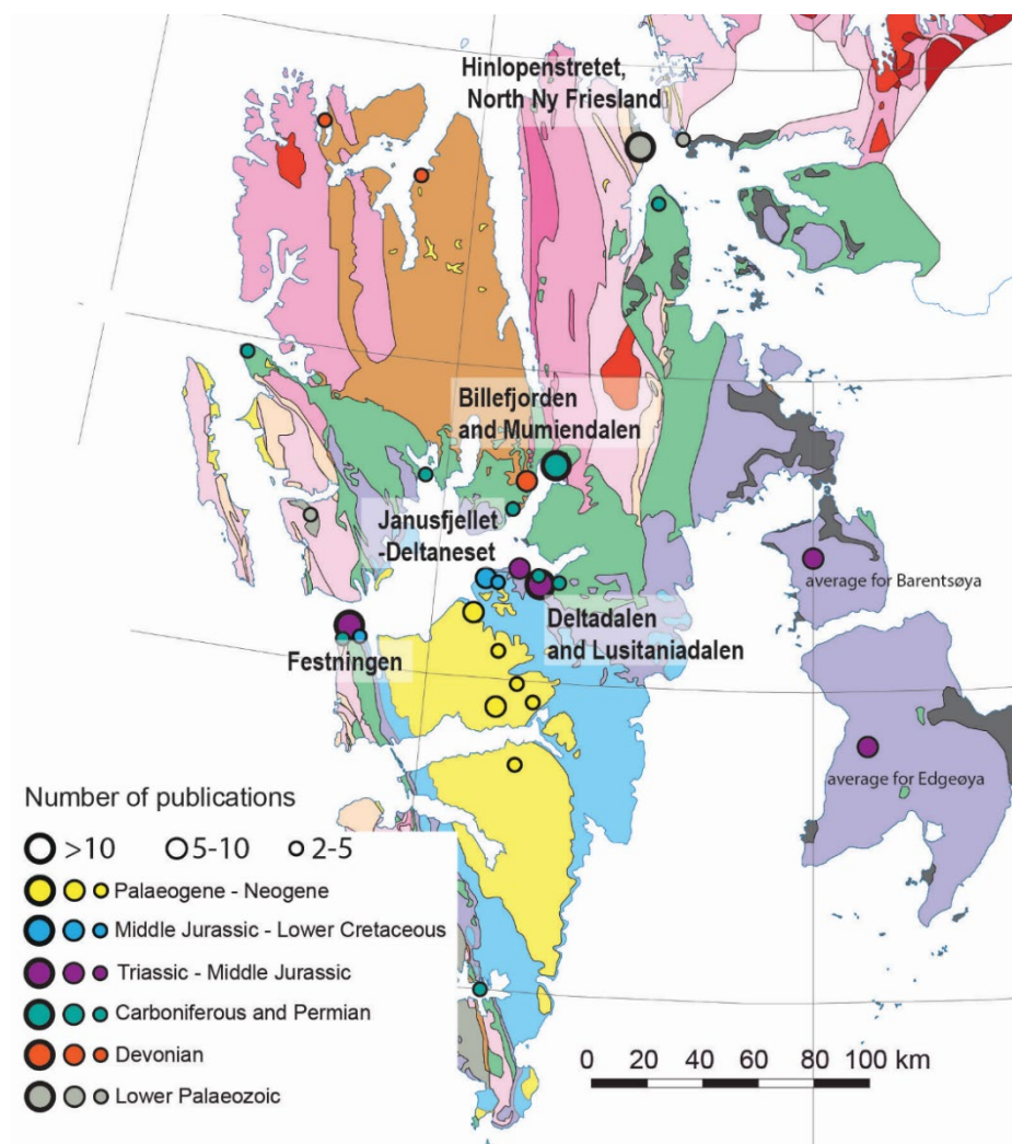
Figure 5: Location of data presented in the reviewed articles summed up in Table A3 (Supplementary table) highlighting the most studied sections in Svalbard. The size of a circle corresponds to the number of publications addressing deep-time paleoclimate proxies. For legend to the geological map see Fig. 2.
