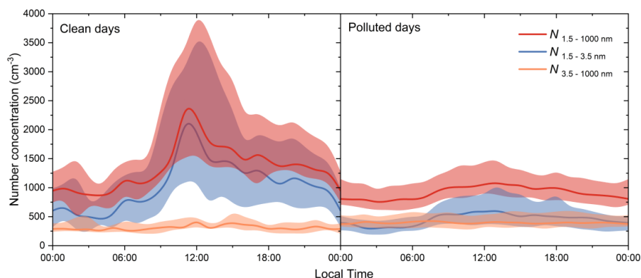
465 Figure 9. Diurnal variation in number concentrations on clean (left panel) and polluted days (right panel) based on PSM measurements for particles with diameters between 1.5 and 1000 nm (red), 1.5 and 3.5 nm (blue) and 3.5 and 1000 nm (orange). The Lines indicate median values and the shaded areas indicate the 25th-75th percentiles.
