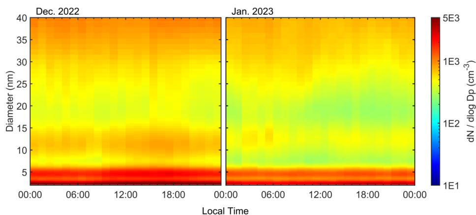
455 Figure 7. Diurnal variation of the particle number size distribution measured by NAIS during December 2022 (left panel) and January 2023 (right panel). The plot data represent the median values.
