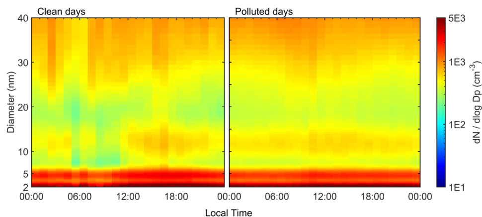
470 Figure 10. Diurnal variation of the particle number size distribution measured by NAIS during clean days (left panel) and polluted days (right panel). The plot data represents the median values.
