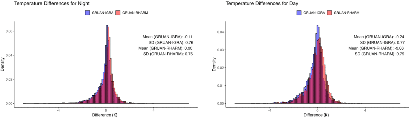
Figure 3: Histogram of night-time (left) and daytime (right) temperature differences between IGRA and GRUAN (blue) and between RHARM and GRUAN (red) at 10 hPa at 8 GRUAN stations (Cabauw, Lamont, Lauder, Lindenberg, Ny-Ålesund, Payerne, Sodankyla, and Tenerife) where RS92 GRUAN data product version 2 is available for the period from 2008 to 2018. All the available ascents have been considered. Note that the starting and ending dates are different at different stations, depending on the sonde type transition date at each station. For example, in 2008, there were only two stations, Lindenberg and Ny-Ålesund. The high-resolution GRUAN RS92 data (at 10 m) were matched with IGRA and RHARM data, that are available only at mandatory and significant levels through a linear interpolation, of levels using the two nearest levels, respectively, above and below 10 hPa. The bias between GRUAN data and RHARM data as well as the random uncertainty for both data sets are discussed in Madonna et al. (2022).
