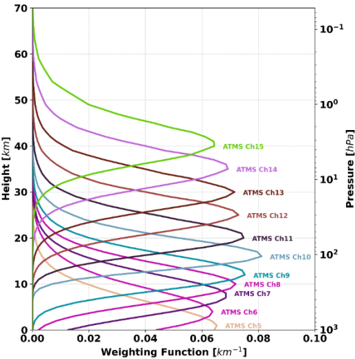
Figure 7: Weighting functions for temperature-sensitive ATMS channels 5 to 15, computed at 1km resolution (adapted from Zou et al., 2018). These show that channel 13 has the largest sensitivity in the region of interest, peaking between 10-20 hPa. Weighting functions of channels 14 and 15 peak higher in the atmosphere, indicating lower sensitivity to the region below 10 hPa.
