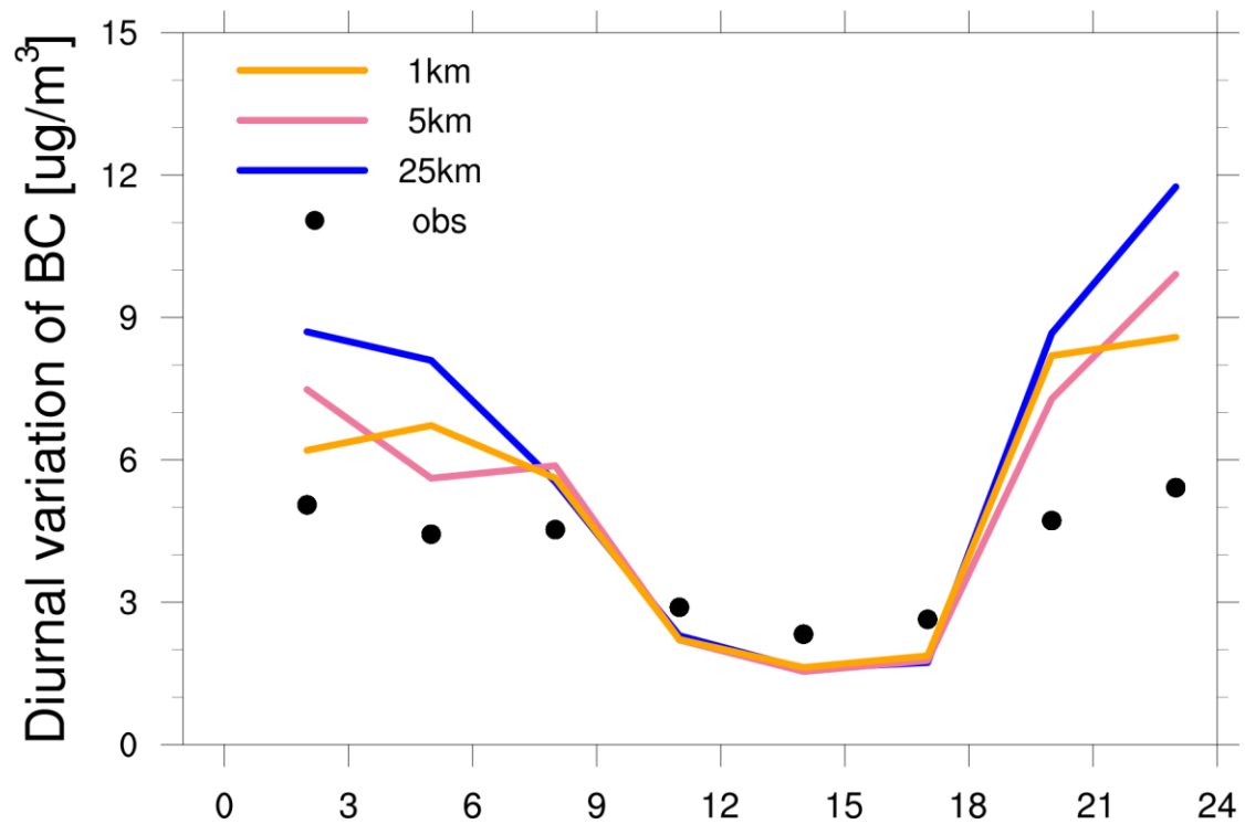
1543 Figure 5. Diurnal variation of BC surface concentrations within 24 h averaged over 1544 the USTC site during the study period for 25-km (solid blue line), 5-km (solid pink 1545 line), and 1-km (solid orange line) resolution simulations and observations (black 1546 dot). Both the simulated results and observations are sampled at the model output 1547 frequency, i.e., 3-hourly.
