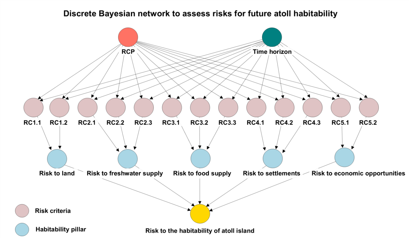
Figure 5 Bayesian network developed for Malé atoll Island.
