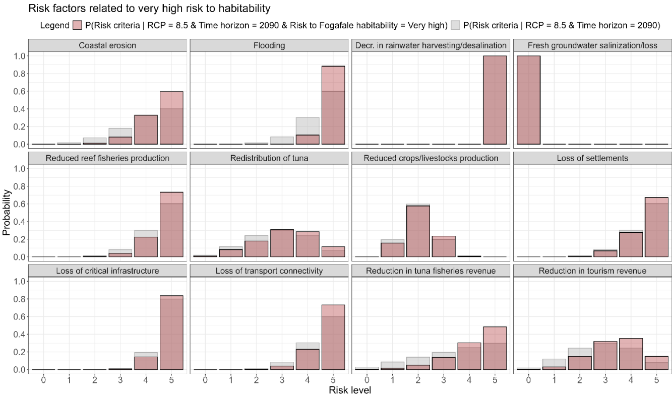
Figure 9 Probability of risk criteria levels under the RCP 8.5 in 2090. The red bars represent the results when the risk to Fogafale habitability is very high (query: P(Risk criteria | RCP = 8.5 & Time horizon = 2090 & Risk to Fogafale habitability = Very high)). The grey bars represent the results without the habitability constraint (query: P(Risk criteria | RCP = 8.5 & Time horizon = 2090)). The results reflect which risk criteria are associated with high risk to Fogafale habitability. These include flooding, loss of critical infrastructure, reduced reef fisheries production and decrease in rainwater harvesting.
