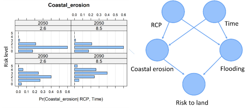
130 Figure 3 Example of a BN structure composed of five nodes (right) and a CPT (left) containing the local conditional distribution of the variable Coastal erosion given its parents RCP and Time.
