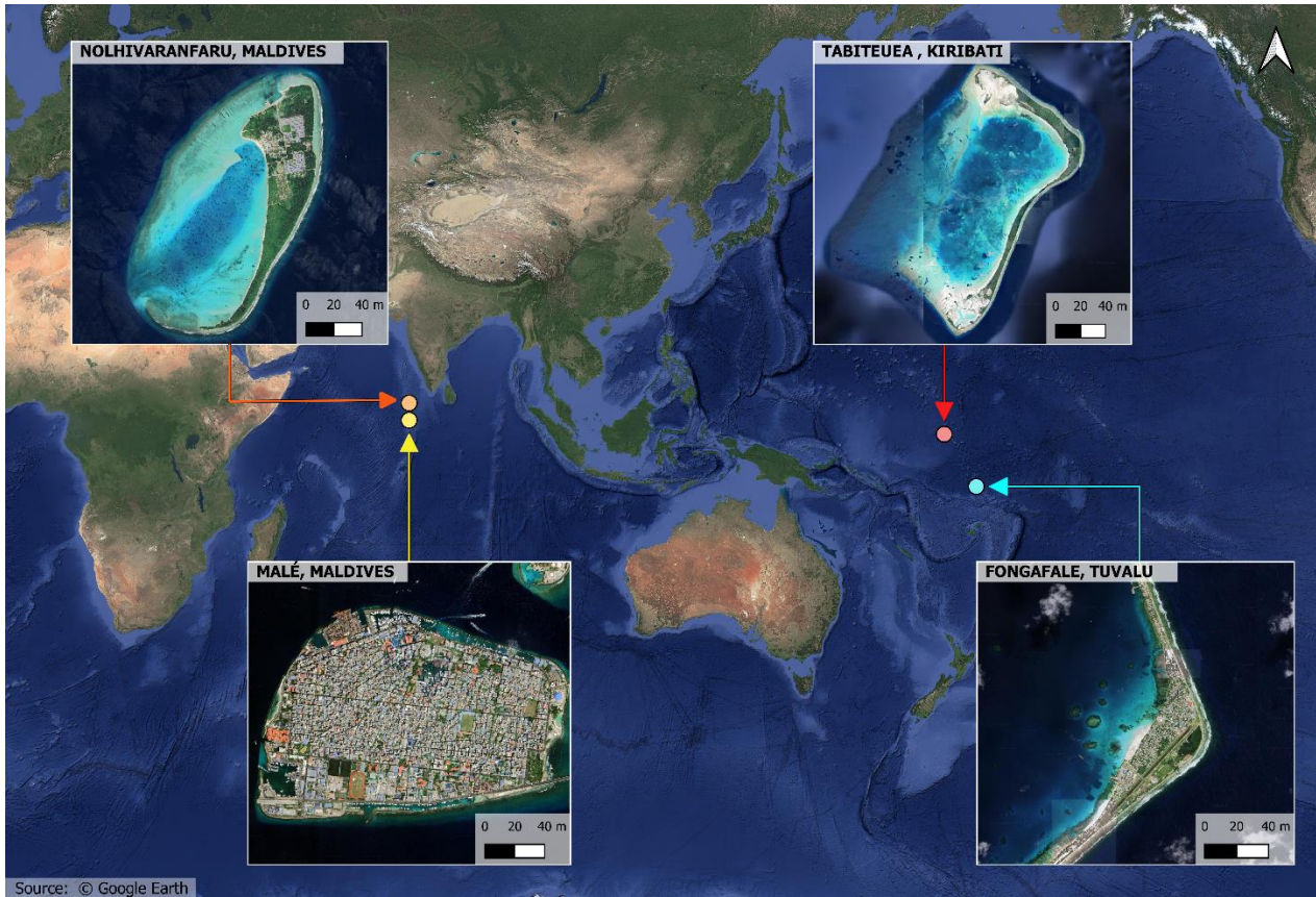
Figure 1 Location of the atoll islands of interest: Malé and Nolhivaranfaru in the Indian Ocean, and Fogafale and Tabiteuea in the Pacific Ocean.
