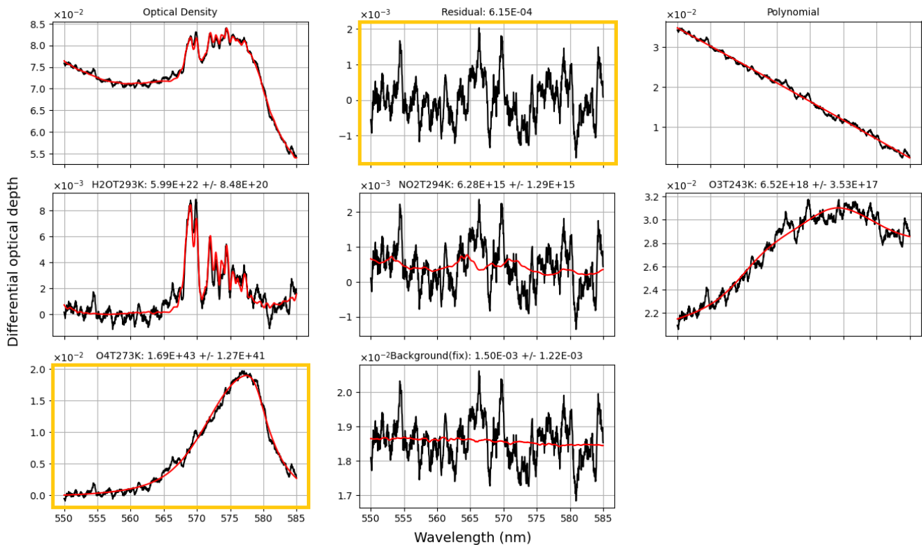
Figure A1. Example fit in the visible spectral range using the fit settings given in Table A1. For the plot description, see Fig. 4.
