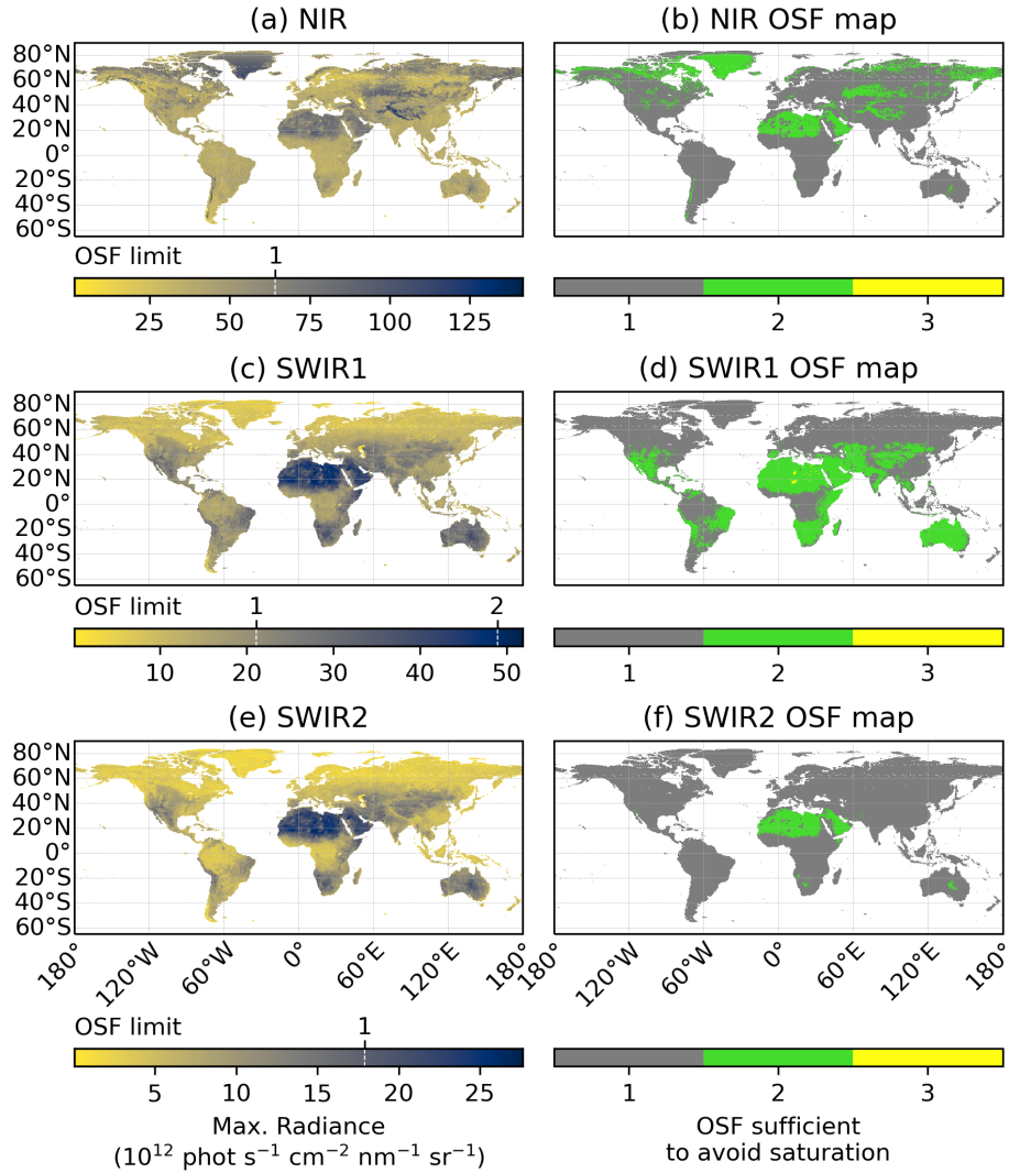
Figure 2. Left column: spectral and temporal maximum radiance in the simulated 1-year subset nadir radiances, binned to a 0.4x0.4 degree latitude-longitude grid. Clouds are removed for this analysis. The radiance limits corresponding to the OSFs in each wavelength band are illustrated by white dashed lines in the color scales of the panels. Right column: OSF needed in order to avoid saturation for the maximum radiances. The rows show the wavelength bands of CO2I: a, b NIR; c, d SWIR1 and e, f SWIR2. The simulated radiances are for nadir over land, only. Therefore, the ocean is masked by white color.
