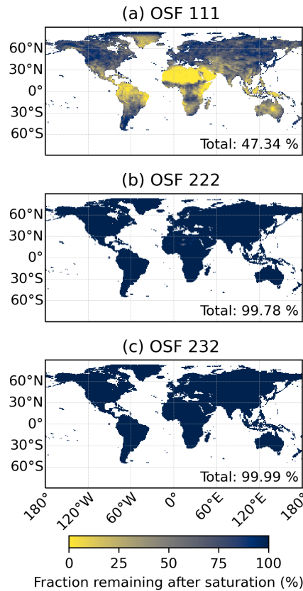
Figure B1. Same as left column of Fig. 5, but removing whole swaths instead of single spatial samples.
