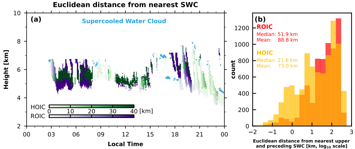
Figure 10. (a) The time-height cross-section of the Euclidean distance between the HOICs, ROICs, and supercooled water cloud bins on 13 Oct. 2022. The light blue range bins represent the supercooled water cloud bins. The color indicates the Euclidean distance; the darker the color (dark green and dark purple), the farther the Euclidean distance. Note here we use a green colorbar instead of orange for HOICs and a purple colorbar instead of red for ROICs to better discriminate HOIC and ROIC with different lightness of color. (b) The histogram of the Euclidean distance between the HOICs, ROICs, and supercooled water cloud bins on 13 Oct. 2022 in \log_{10} scale with the median and mean value noted in the upper left corner.
