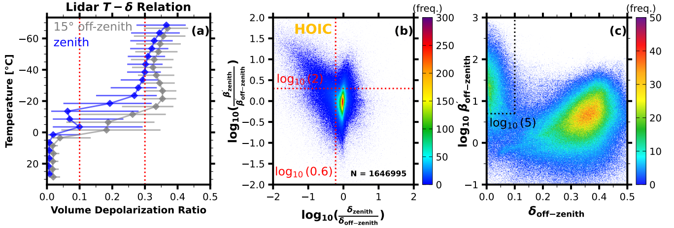
Figure 3. Definition of criteria for identification of the HOICs (red dashed lines). All subfigures were created using all the cloud bins observed in 2022. (a) Median volume depolarization ratio as a function of temperature for each height bin within all detected cloud bins in temperature increments of 5 °C. Horizontal bars indicate the interquartile range (IQR). (b) Density scatter plot of the ratio of zenith- to off-zenith-pointing lidar’s volume depolarization and attenuated backscatter, \log_{10} scale. (c) Density scatter plot of volume depolarization ratio and attenuated backscatter (unit in \text{Mm}^{-1}\text{sr}^{-1} , \log_{10} scale) for off-zenith-pointing lidar. Black dashed lines indicate the criteria used for the identification of liquid water.
