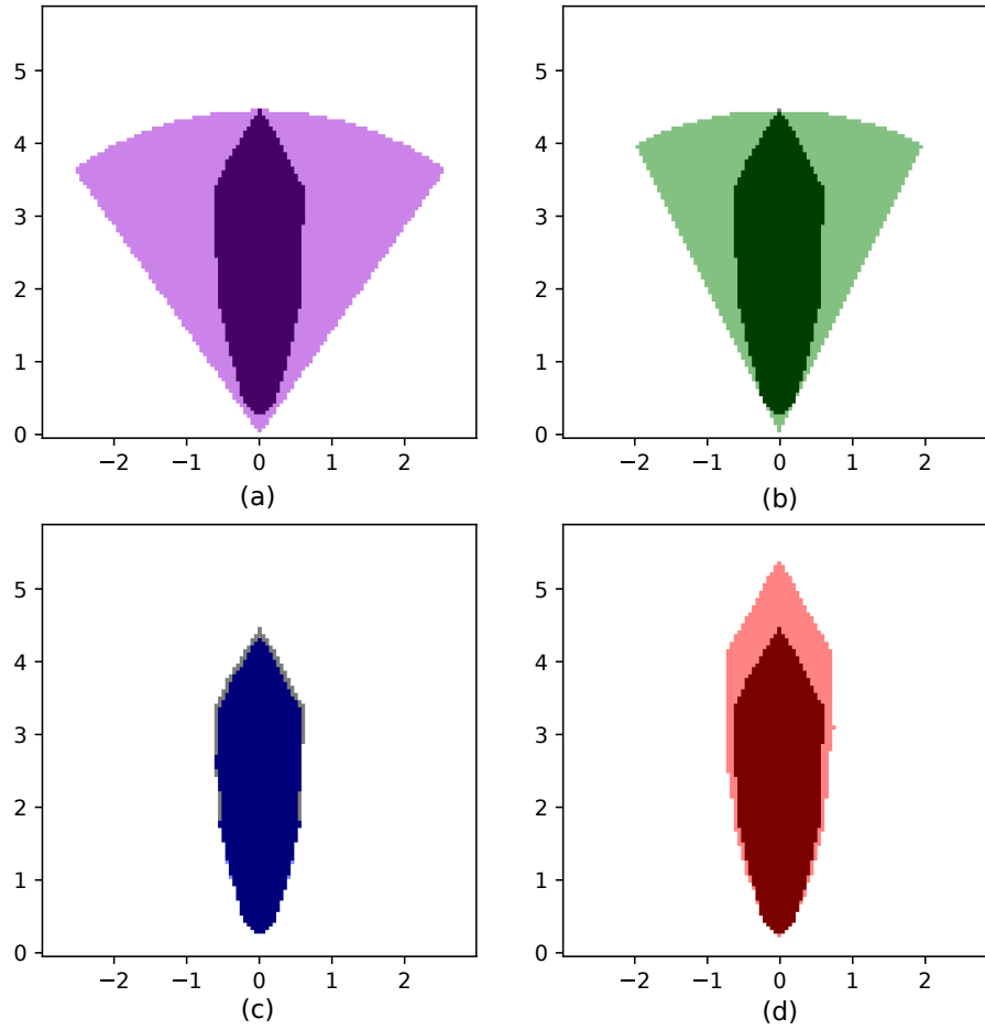
Figure 8. Guide-level exceedance zone, for one simulation of the test sample, obtained by the different estimation methods. Each subfigure corresponds to a different method: (a) the ATS estimator (in purple), (b) the emulator of geometrical parameters (in green), (c) the emulator coupling Kriging to AAM (in blue), and (d) the same emulator with a lower threshold (in red). In each plot, the estimated exceedance zone is shown in light color, and the reference exceedance zone given by the Gaussian puff model pX is superimposed in grey. Colors are consistent with other figures to ease comparison between methods.
