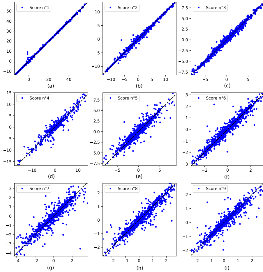
Figure 5. Comparison of the prediction of the emulator (in y-axis) with the target obtained by simulation (in x-axis). Each graph represent one coordinate of the AAM.
