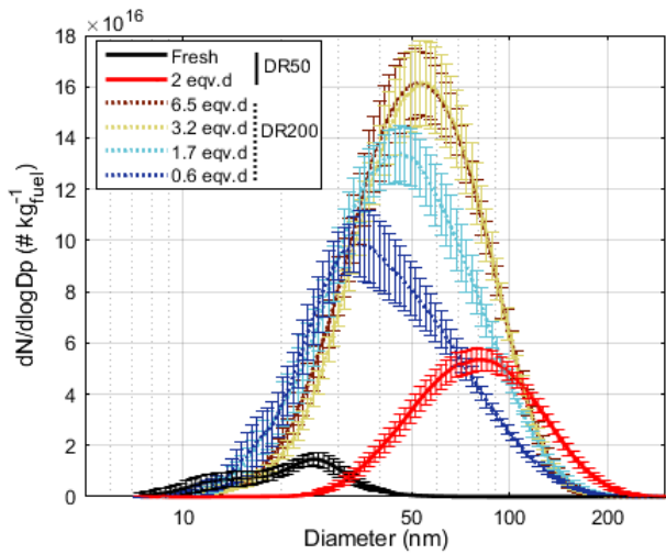
460 Figure 5. Particle number size distributions measured by the SMPS for the fresh and aged exhaust emissions. Error bars denote the standard deviations over the whole experimental time (12 or 16 h for the DR50 fresh and aged experiments, respectively; 40 to 70 min for the DR200 experiments).
