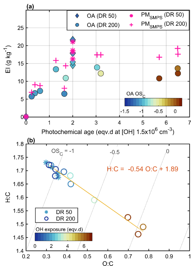
470 Figure 6. Mass emission indices for the particles measured by SMPS ( \text{PM}_{\text{SMPS}} ) and organic aerosol (OA) measured by the AMS, with average carbon oxidation state indicated by color (a), and average elemental ratios of the organic aerosol, with OH exposure indicated by color (b).
