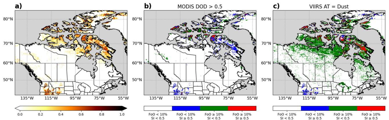
Figure 6. a) Source intensity (SI) from the G-SDS-SBM dataset for July. b) Combined classification map based on SI and FoO MODIS DOD PG16 > 0.5 as a percentage of the number of DOD PG16 retrievals available; c) Combined classification map based on SI and FoO VIIRS AT DUST as a percentage of the number of VIIRS Aerosol Type (AT) retrievals available. Grey shading indicates no data.
