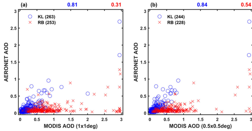
Figure 8. Maximum AERONET AOD (500 nm) between 11 am and 5 pm local time at Kluane Lake (blue open circles) and Resolute Bay (red crosses) vs. maximum MODIS AOD from a) a 1^\circ \times 1^\circ box centred on each station; b) from b) a 0.5^\circ \times 0.5^\circ box centred on each station. Numbers in blue (red) above each panel correspond to the Pearson's correlation coefficient, R , between Kluane Lake (Resolute Bay) AERONET AOD and the MODIS dataset in that panel. The number of matched maximum AOD days for each comparison is given in parentheses in the legends.
