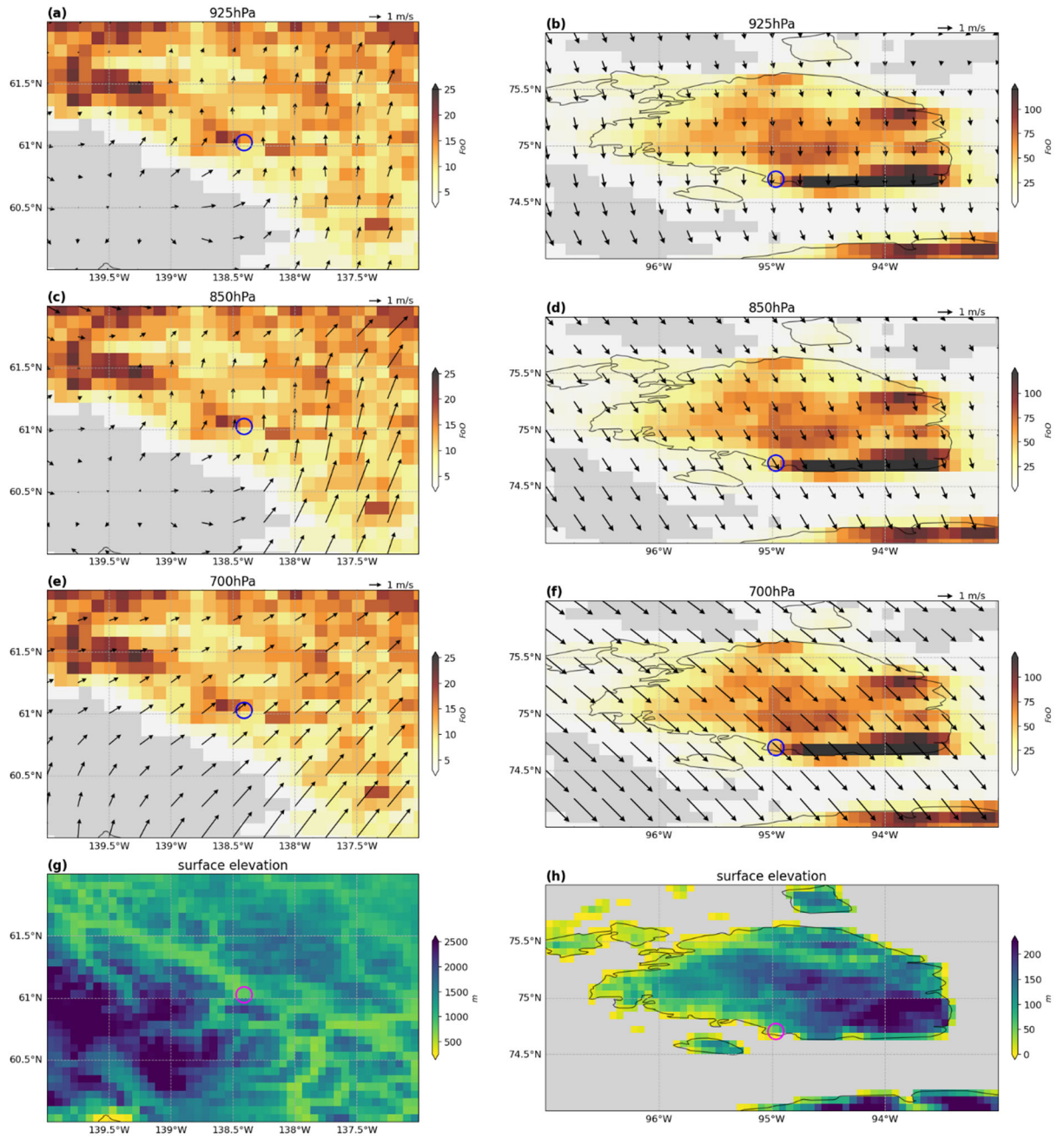
Figure 10. a,c,e) Winds at 925 hPa, 850 hPa, and 700 hPa above the region surrounding the Kluane Lake AERONET station (blue circle). Winds are the mean of ERA-5 reanalysis data for Jun 07 – Aug. 2004 – 2023. Underlying shading corresponds to FoO DOD PG16 > 0.5 for the period 2003 – 2022 (grey shading corresponds to no data). g) Surface elevation surrounding Kluane Lake station (red circle) at 0.0625 degrees resolution from the Global Multi-resolution Terrain Elevation Data 2010 (GMTED2010) dataset. b,d,f,h) Like a,c,e,g) except for Resolute Bay AERONET station.
