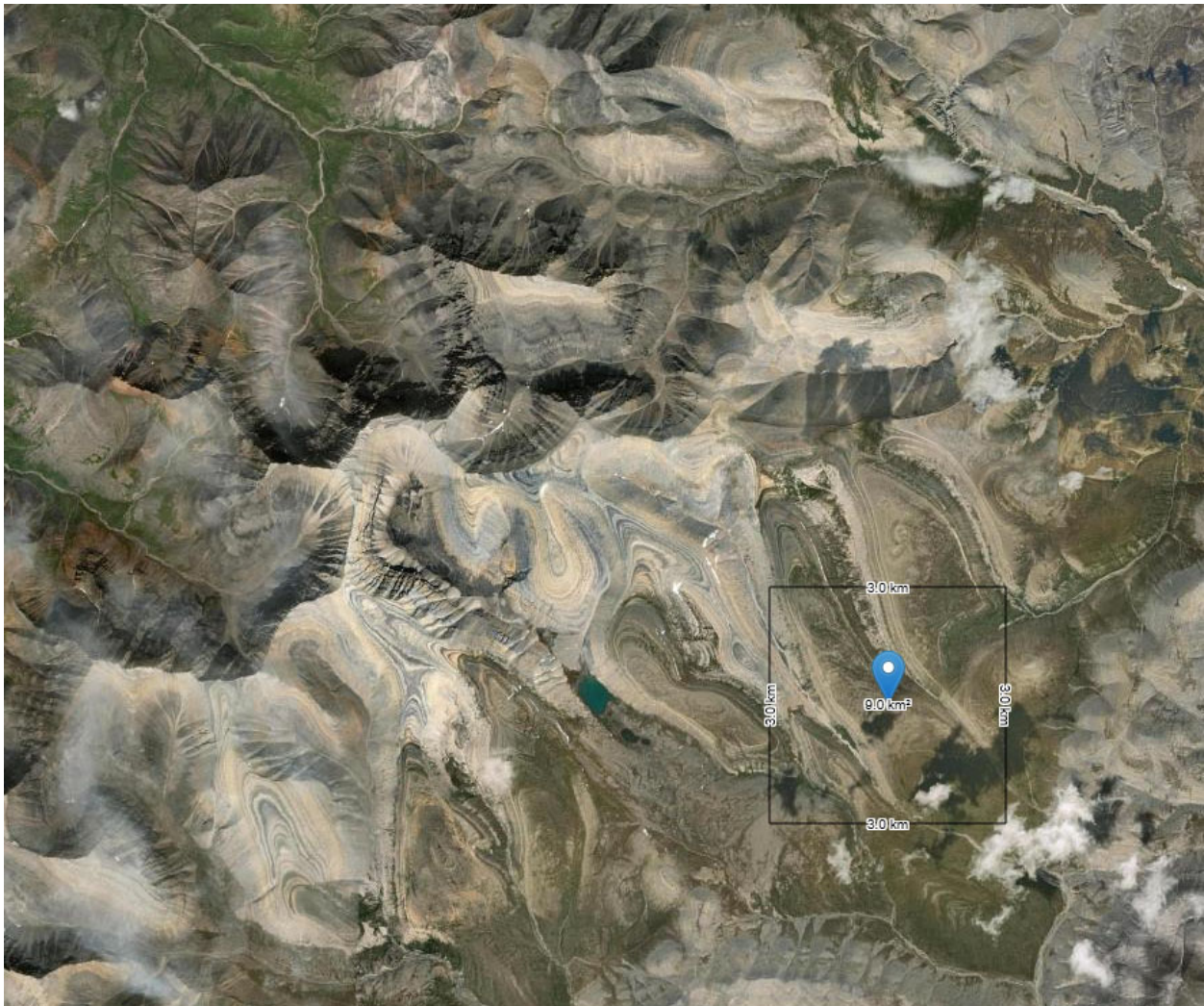
715 Figure A1. Visible imagery of the dust emission source area in the MacKenzie Mountains (marked by a pink square in Fig. 11). Centre of 9.0 km 2 box is at 63°N, 126°W with a mean wind speed of 8.13 m/s (predominantly westerly). Topography varies from 900 m to 2300 m in full region shown. Obtained from the Global Wind Atlas version 3.3, a free, web-based application developed, owned and operated by the Technical University of Denmark (DTU). The Global Wind Atlas version 3.3 is released in partnership with the World Bank Group, utilizing data provided by Vortex, using funding provided by the 720 Energy Sector Management Assistance Program (ESMAP). For additional information: https://globalwindatlas.info . 10-m resolution Google visible imagery is available at, e.g., 63.16920, -126.09163 (the precise location above is snow-covered).
