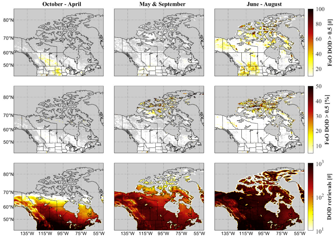
Figure 3. Seasonal cycle in \text{FoO DOD}_{\text{PG16}} \geq 0.5 over Canada (MODIS data spans 2003 – 2022). Top row) \text{FoO DOD}_{\text{PG16}} > 0.5 , by season. Middle row) \text{FoO DOD}_{\text{PG16}} > 0.5 as a percentage of the number of \text{DOD}_{\text{PG16}} retrievals, by season. Bottom row) number of \text{DOD}_{\text{PG16}} retrievals, by season. Left column) October – April inclusive (winter season). Middle column) May and September (shoulder season). Right column) June – August inclusive (summer season). Grey shading corresponds to no data.
