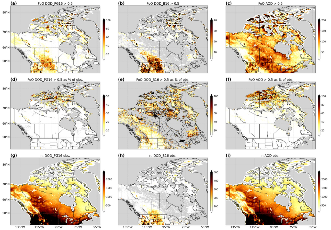
Figure 1. Frequency of Occurrence (FoO) of a) \text{DOD}_{\text{PG16}} > 0.5 , b) \text{DOD}_{\text{B16}} > 0.5 , and c) \text{AOD} > 0.5 . FoO as a percentage of the number of retrievals available d) \text{DOD}_{\text{PG16}} > 0.5 , e) \text{DOD}_{\text{B16}} > 0.5 , and f) \text{AOD} > 0.5 , with corresponding g) \text{DOD}_{\text{PG16}} , h) \text{DOD}_{\text{B16}} , and i) \text{AOD} . Note the different colour scales used. Grey shading corresponds to no data. All panels are based on MODIS data for 2003 – 2022.
