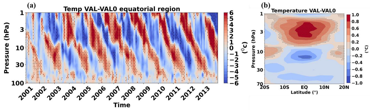
Fig.: (a) Time series of temperature zonally averaged over the 5S-5N for the period 2001-2013. (b) Latitude-pressure cross section of zonally averaged temperature for period 2001-2013 from VAL-VAL0 simulation. The black dots indicate the regions where the differences are significant for the difference of the mean (p-value < 0.05) using a two-sided t-test.
