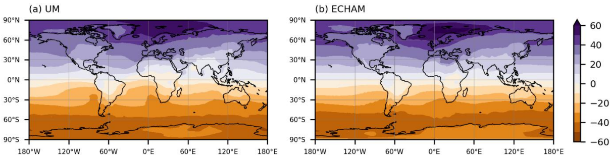
345 Figure 5: Mass-weighted mean of the evaporative source latitude (in degrees) of annual mean ocean-sourced precipitation for: a) UM; and b) ECHAM6.
