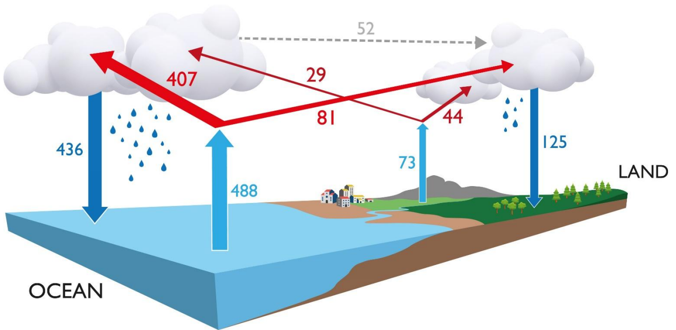
370 Figure 8: Global hydrological cycle fluxes (in 10^3 \text{ km}^3 \text{ yr}^{-1} ) derived from the prescribed region water tracer precipitation fields. The 375 separate land and ocean sources of both the annual mean land and ocean precipitation are shown from the model simulation (1985- 2014). The red arrows indicate the additional information provided by the water tracers compared to standard diagnostics. The grey dashed arrow shows the net ocean to land flux of atmospheric water. Sea ice is included in the ocean component for this diagram.
