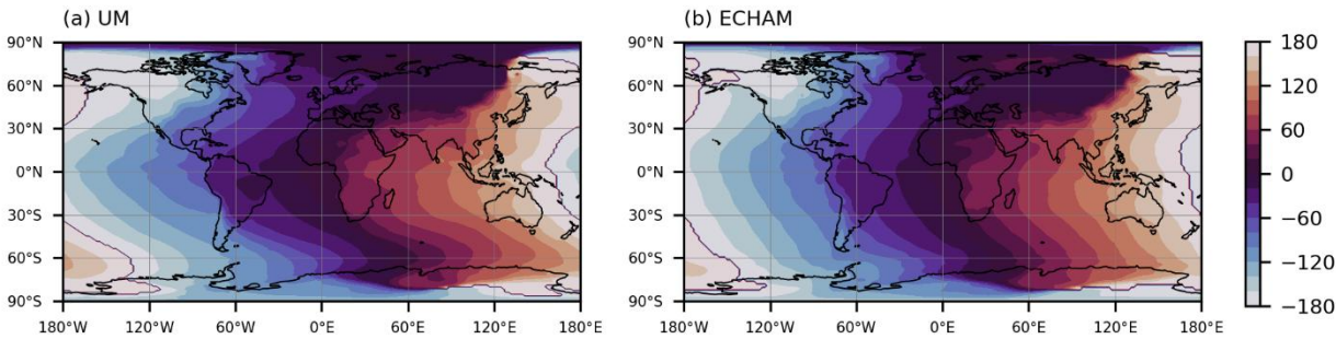
350 Figure 6: Mass-weighted mean of the evaporative source longitude (in degrees) of annual mean ocean-sourced precipitation for: a) UM; and b) ECHAM6.
