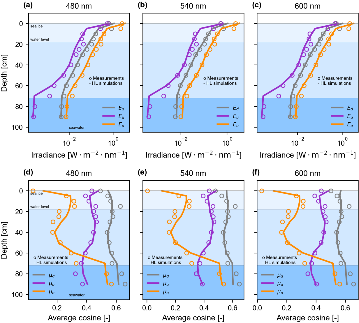
855 Figure S1: Vertical profiles of all irradiance quantities (planar downward, planar upward, and scalar) measured and simulated in the 480 nm (a), the 540 nm (b), and the 600 nm (c) spectral channels. In the same order of wavelengths, the second row shows the average cosines (planar downward, planar upward, and scalar) as a function of depths across the different boundaries measured during the fieldwork.
