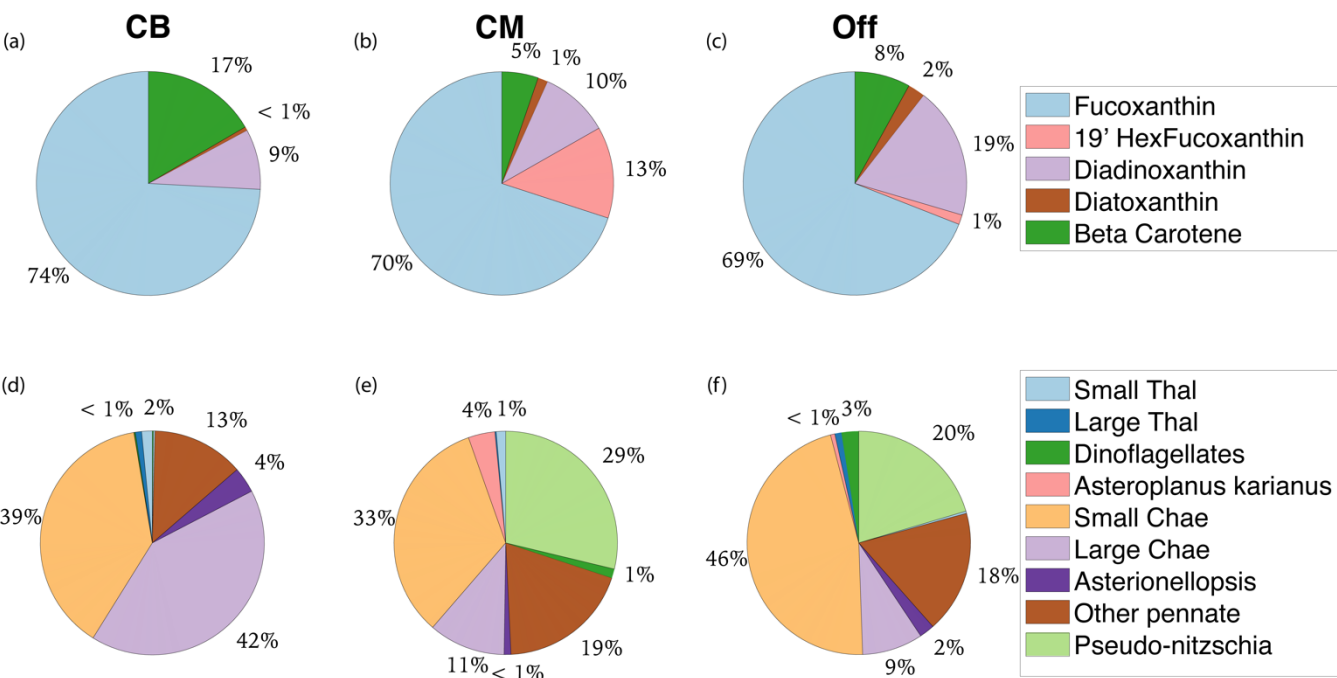
965 Figure B1. Pigment and taxonomic composition of study area sub-regions. a-c) display non-Chl pigment distribution by mass for Cape Blanco (CB), Cape Mendocino (CM), and Offshore (Off). d-f) display the taxonomic distribution of diatom and dinoflagellate groups visible for microscope counts.
