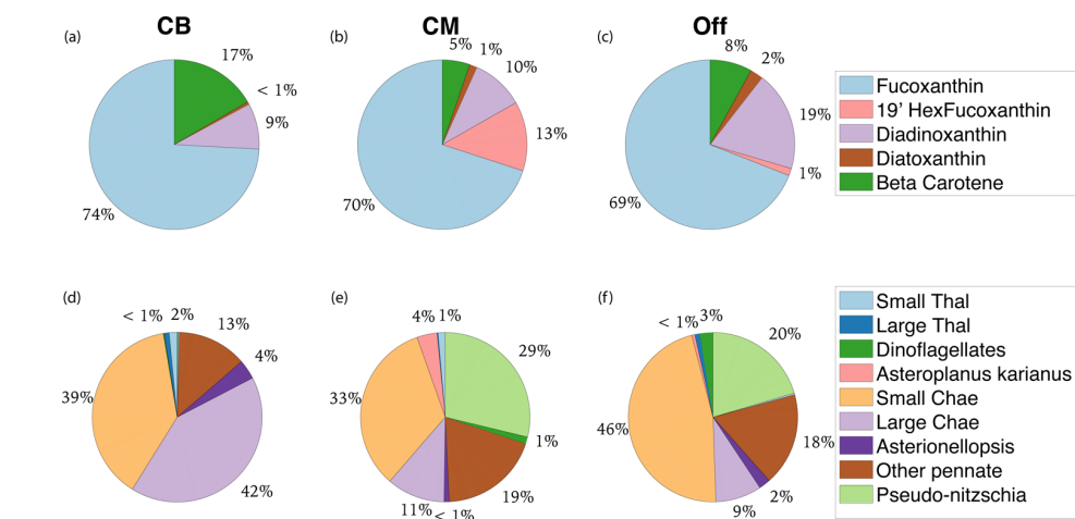
005 Figure B1. Pigment and taxonomic composition of study area sub-regions. a-c) display non-Chl pigment distribution by mass for Cape Blanco (CB), Cape Mendocino (CM), and Offshore (Off). d-f) display the taxonomic distribution of diatom and dinoflagellate groups visible for microscope counts.
