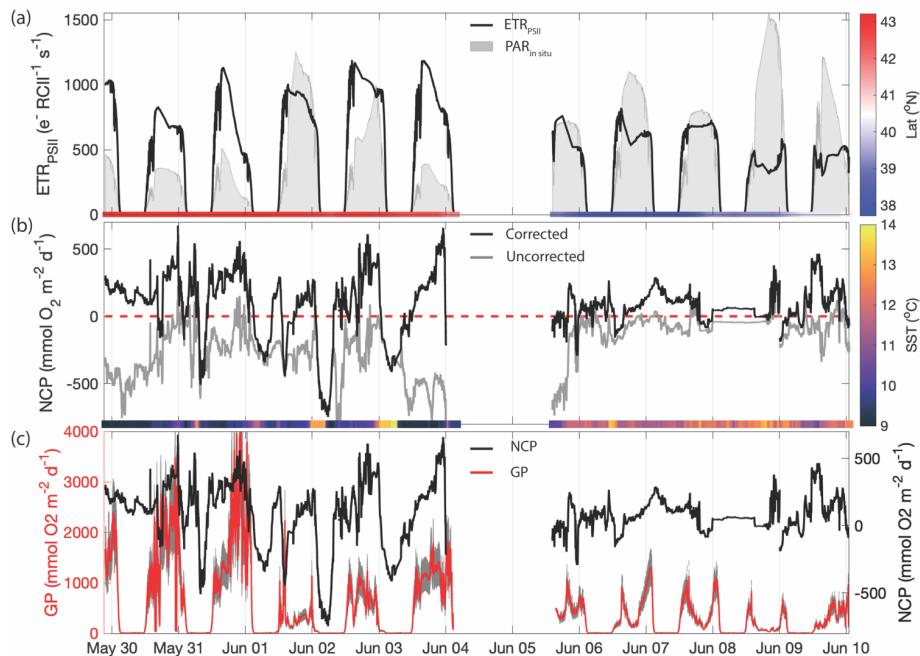
540 Figure 5. Primary productivity time series along the cruise track. a) ETR_{PSII} derived from FRRF- measured PI curve parameter interpolated to match NCP sampling frequency (black line). The grey patches indicate the mean PAR available within the mixed layer ( PAR_{in situ} ). The bar on the bottom is coloured by the sampling latitude. The Cape Blanco filament is designated as latitude > 40.5 and is coloured red, while Cape Mendocino is designated as latitude < 40.5 coloured blue. b) Uncorrected 545 NCP (grey) and mixing-corrected NCP (black). The dashed red line denotes the boundary between net autotrophy ( NCP > 0 ) and net heterotrophy ( NCP < 0 ). The color bar on the bottom illustrates the sample temperature. c) mixing-corrected NCP (black, right y-axis) and gross photochemistry (GP), shown in red (left y-axis). GP is calculated by converting ETR_{PSII} from units e^- RCII^{-1} s^{-1} to mmol O_2 m^{-2} d^{-1} . The grey shading around the red line displays the range of GP based on an assumed range of 400 – 550 700 Chl:RCII .
