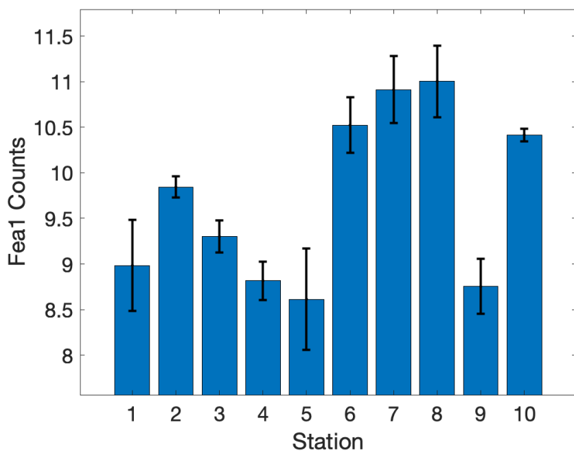
010 Figure C1. Diatom-specific expression of Fe assimilation gene Fea1 . Bar height displays the mean of normalized Fea1 counts mapping to Bacillariophyta by station. Normalized Fea1 counts were calculated using DESeq2's median of ratios method in R (Love, Huber, and Anders 2014). Error bars display the standard deviation. Stations 1-4 were in close proximity of Cape Blanco, 6 and 10 were offshore while the remaining stations were in proximity of the Cape Mendocino upwelling filament.
