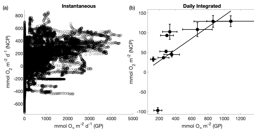
Figure 9. Comparison between fluorescence-based gross photochemistry (GP) and NCP. Panel (a)
