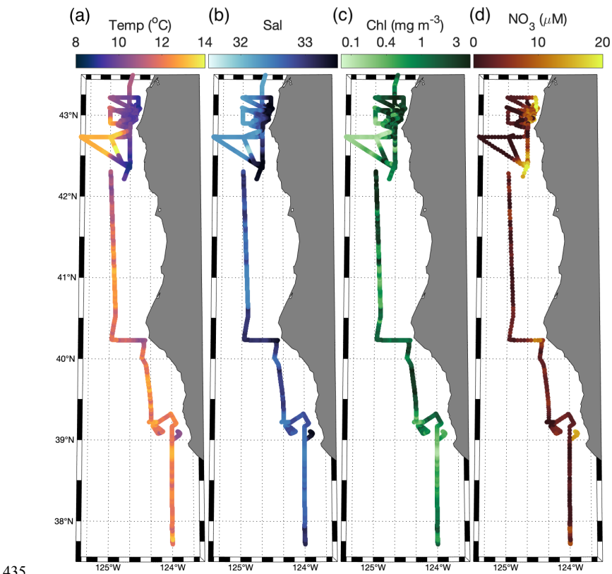
435 Figure 2. Surface water (a) SST, (b) salinity, (c) Chl, and (d) \text{NO}_3^- along the cruise track. Cape Mendocino is abbreviated as Cape Mendo.
