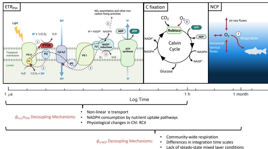
775 Figure 7. Different primary productivity currencies and their decoupling mechanisms. The three productivity currencies of interest are indicated with respect to the times scales they represent. Numbered red pathways denote decoupling mechanisms including 1) chloro-respiration 2) cyclic transport around PSII 3) cyclic transport around PSI 4) pseudo-cyclic/ Mehler reactions 5) reductant consuming nutrient uptake pathways 6) photo-respiration and 7) Community-wide respiration. Figure 780 produced in Biorender.
