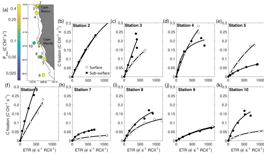
Figure 6. Parallel measurements of fluorescence- and ^{14}\text{C} -based photosynthesis-irradiance experiments conducted on-station. The top left displays the sample locations coloured by maximum
