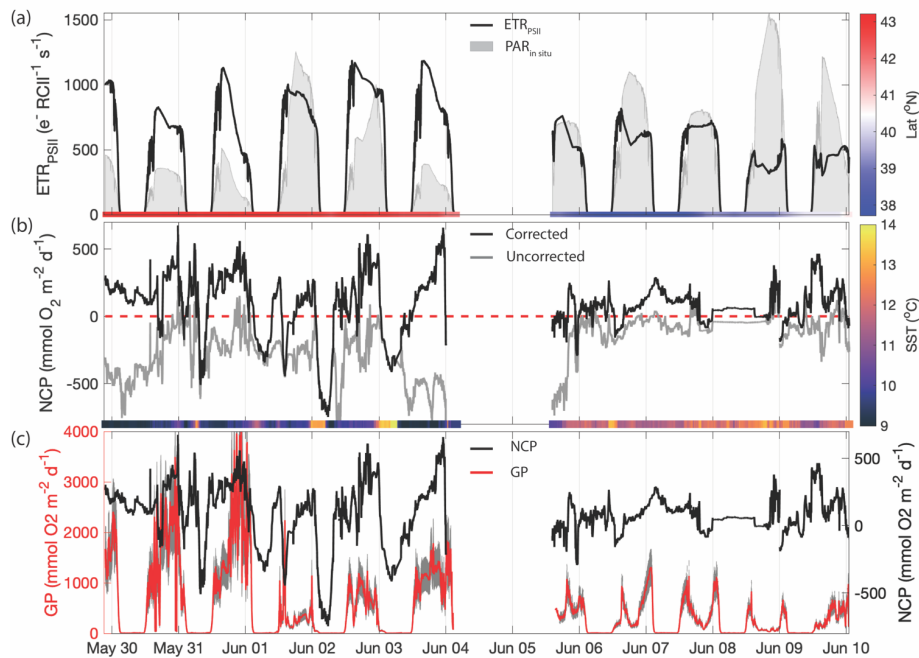
595 Figure 5. Primary productivity time series along the cruise track. a) ETR_{PSII} derived from FRRF-measured PI curve parameter interpolated to match NCP sampling frequency (black line). The grey patches indicate the mean PAR available within the mixed layer ( PAR_{in situ} ). The bar on the bottom is coloured by the sampling latitude. The Cape Blanco filament is designated as latitude > 40.5 and is coloured red, while Cape Mendocino is designated as latitude < 40.5 coloured blue. b) Uncorrected NCP (grey) and mixing-corrected NCP (black). The dashed red line denotes the boundary between net autotrophy ( NCP > 0 ) and net heterotrophy ( NCP < 0 ). The color bar on the bottom illustrates the sample temperature. c) mixing-corrected NCP (black, right y-axis) and gross photochemistry (GP), shown in red (left y-axis). GP is calculated by converting ETR_{PSII} from units e^- RCII^{-1} s^{-1} to mmol O_2 m^{-2} d^{-1} . The grey shading around the red line displays the range of GP based on an assumed range of 400 – 700 Chl:RCII.
