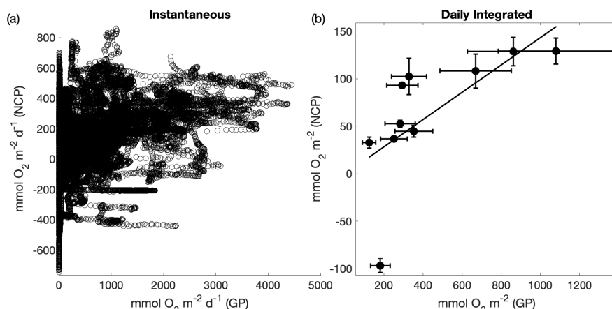
Figure 9. Comparison between fluorescence-based gross photochemistry (GP) and NCP. Panel (a) compares continuous underway ETR PSII and NCP measurements ( \rho = 0.43 , p < 0.01 ), panel (b) compares daily-integrated measurements of ETR PSII and NCP measurements ( \rho = 0.92 , p < 0.01 ). A line of best fit ( y = 0.14 * GP - 0.55 ) is drawn through the positive NCP data points. The error bars represent the total uncertainty of each measurement determined by propagating uncertainty in each input variable. For GP, total uncertainty is represented as the uncertainty in the Chl:RCII. For NCP, uncertainty was quantified from uncertainty in the deep water supply ratio of O 2 :N 2 O, and modelled differences between [N 2 ] and [Ar]. Assumption biases (e.g. no horizontal advection of O 2 ) also represents a potential large source of uncertainty but were not quantified.
