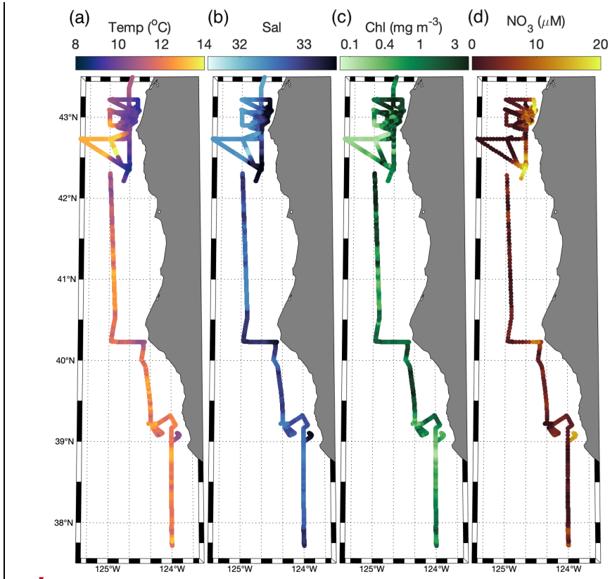
Figure 2. Surface water (a) SST, (b) salinity, (c) Chl, and (d) \text{NO}_3^- along the cruise track. Cape Mendocino is abbreviated as Cape Mendo.
